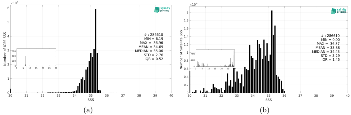
Figure 3: Histograms of SSS from ICES (a) and Aquarius SSS L3 OR v5 - 7-Day running - Rain mask (NASA-GSFC) (b) considering all match-up pairs per bins of 0.1 over the SMOS coastal zone (<800km) 60N-60S Pi-MEP region and for the full satellite product period.
