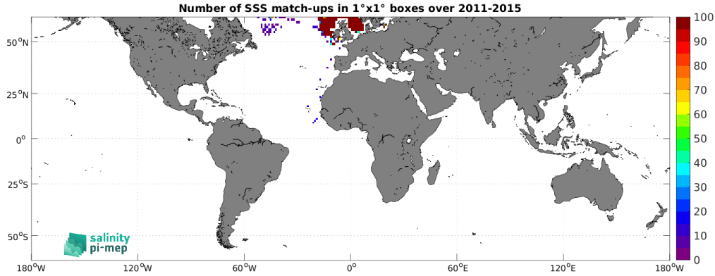
Figure 5: Number of SSS match-ups between ICES SSS and the Aquarius SSS L3 OR v5 - 7-Day running - Rain mask (NASA-GSFC) SSS product for the SMOS coastal zone (<800km) 60N-60S Pi-MEP region over 1^\circ \times 1^\circ boxes and for the full satellite product period.
