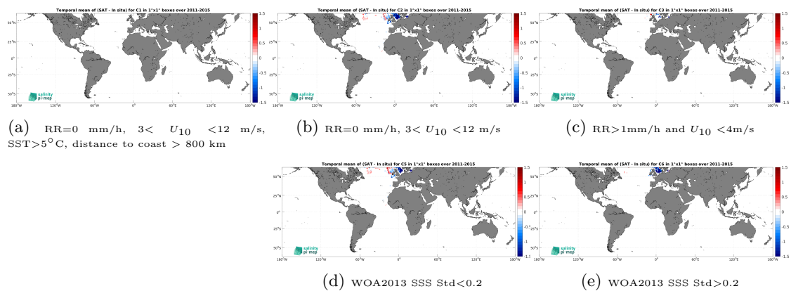
Figure 14: Temporal mean gridded over spatial boxes of size 1^\circ \times 1^\circ of \Delta SSS (Aquarius SSS L3 OR v5 - 7-Day running - Rain mask (NASA-GSFC) - ICES) for 5 different subdatasets corresponding to: RR=0 mm/h, 3 < U_{10} < 12 m/s, SST > 5^\circ\text{C} , distance to coast > 800 km (a), RR=0 mm/h, 3 < U_{10} < 12 m/s (b), RR > 1 mm/h and U_{10} < 4 m/s (c), WOA2013 SSS Std < 0.2 (d), WOA2013 SSS Std > 0.2 (e).
