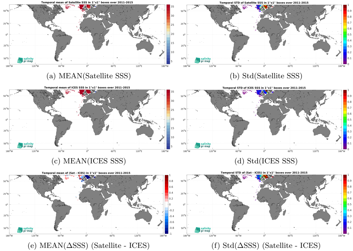
Figure 7: Temporal mean (left) and Std (right) of SSS from Aquarius SSS L3 OR v5 - 7-Day running - Rain mask (NASA-GSFC) (top), ICES (middle), and of \Delta SSS (Satellite - ICES). Only match-up pairs are used to generate these maps.
