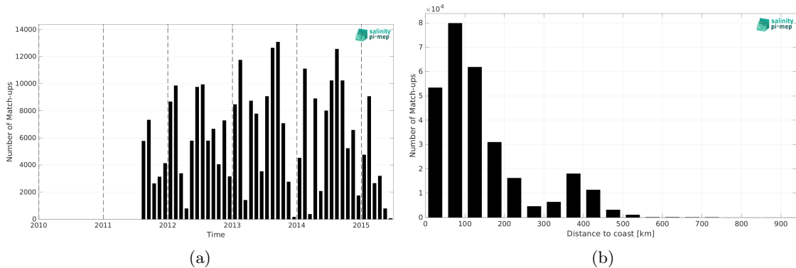
Figure 2: Number of match-ups between ICES and Aquarius SSS L3 OR v5 - 7-Day running - Rain mask (NASA-GSFC) SSS as a function of time (a) and as function of the distance to coast (b) over the SMOS coastal zone (<800km) 60N-60S Pi-MEP region and for the full satellite product period.
