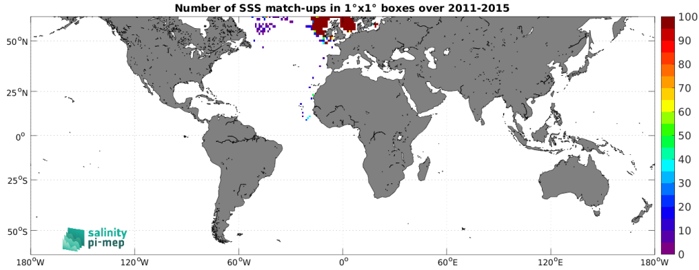
Figure 4: Number of SSS match-ups between ICES SSS and the Aquarius SSS L3 OR v5 - 7-Day running - Rain mask (NASA-GSFC) SSS product for the SMOS coastal zone (<800km) 60N-60S Pi-MEP region over 1^\circ \times 1^\circ boxes and for the full satellite product period.
