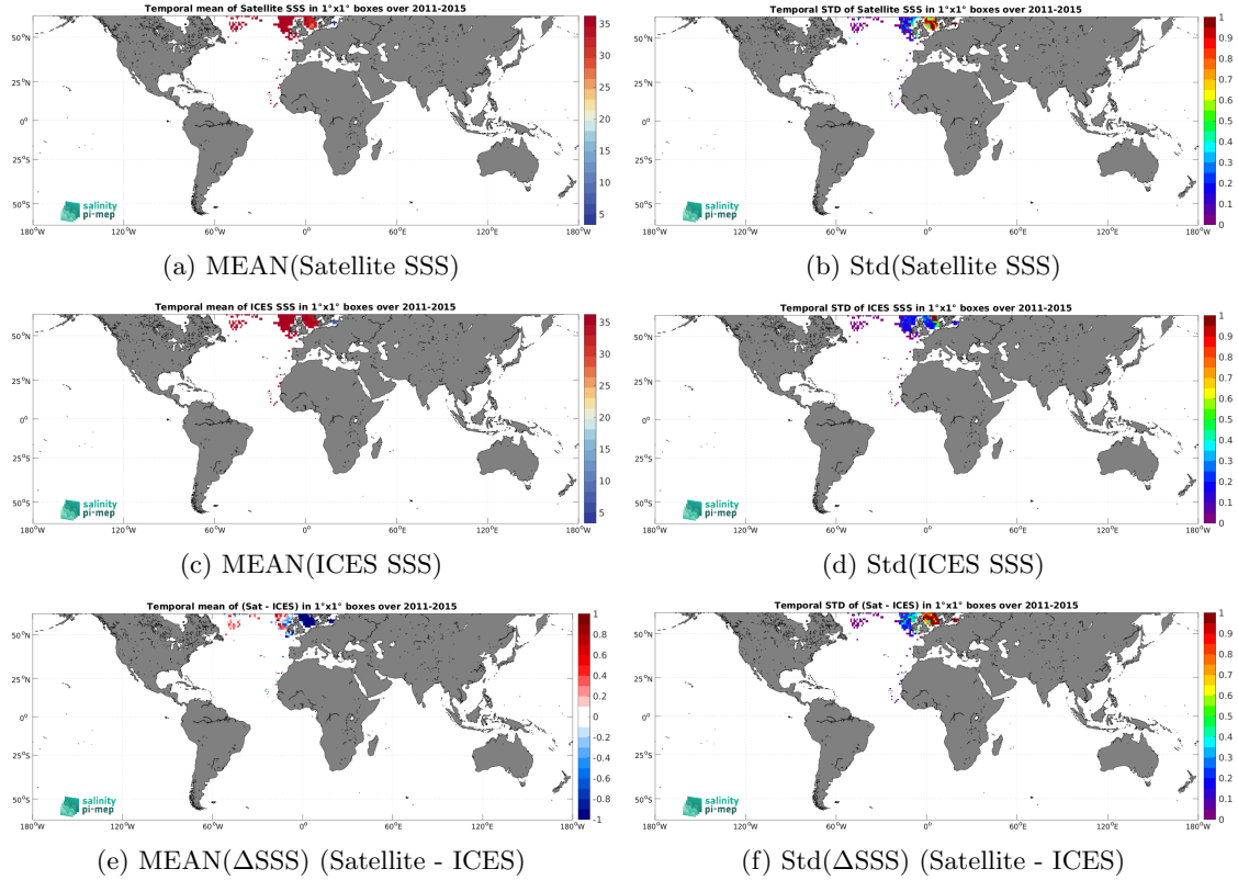
Figure 6: Temporal mean (left) and Std (right) of SSS from Aquarius SSS L3 OR v5 - 7-Day running - Rain mask (NASA-GSFC) (top), ICES (middle), and of \Delta SSS (Satellite - ICES). Only match-up pairs are used to generate these maps.
