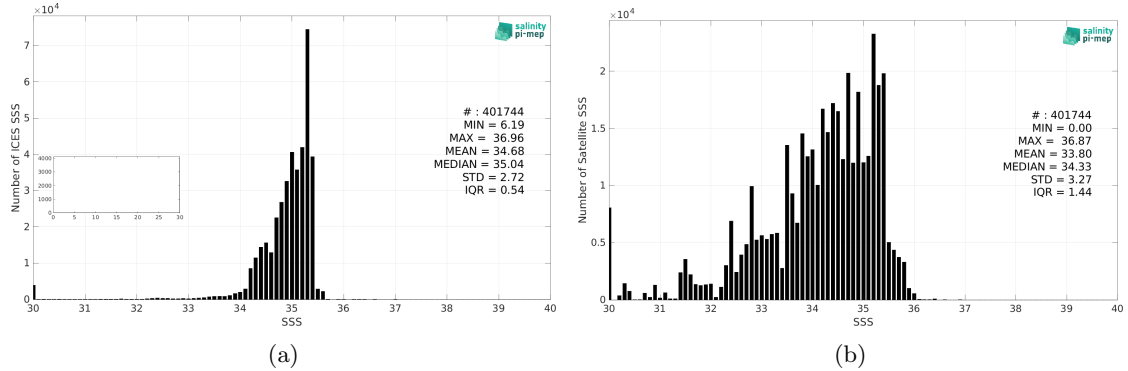
Figure 2: Histograms of SSS from ICES (a) and Aquarius SSS L3 OR v5 - 7-Day running - Rain mask (NASA-GSFC) (b) considering all match-up pairs per bins of 0.1 over the SMOS coastal zone (<800km) 60N-60S Pi-MEP region and for the full satellite product period.
