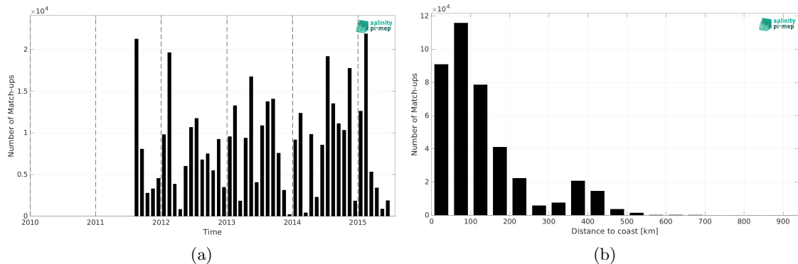
Figure 1: Number of match-ups between ICES and Aquarius SSS L3 OR v5 - 7-Day running - Rain mask (NASA-GSFC) SSS as a function of time (a) and as function of the distance to coast (b) over the SMOS coastal zone (<800km) 60N-60S Pi-MEP region and for the full satellite product period.
