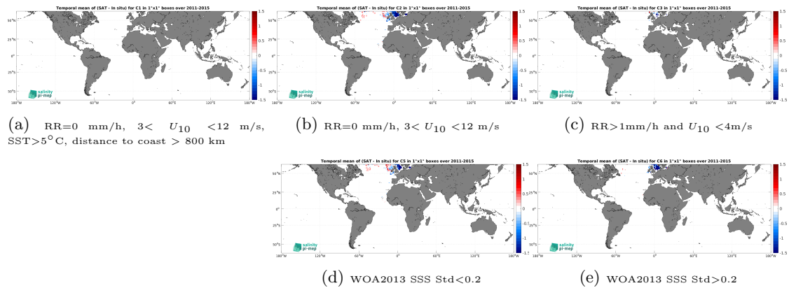
Figure 12: Temporal mean gridded over spatial boxes of size 1^\circ \times 1^\circ of \Delta\text{SSS} (Aquarius SSS L3 OR v5 - 7-Day running - Rain mask (NASA-GSFC) - ICES) for 5 different subdatasets corresponding to:RR=0 mm/h, 3 < U_{10} < 12 m/s, SST >5^\circ\text{C} , distance to coast > 800 km (a), RR=0 mm/h, 3 < U_{10} < 12 m/s (b), RR >1 mm/h and U_{10} < 4 m/s (c), WOA2013 SSS Std <0.2 (d), WOA2013 SSS Std >0.2 (e).
