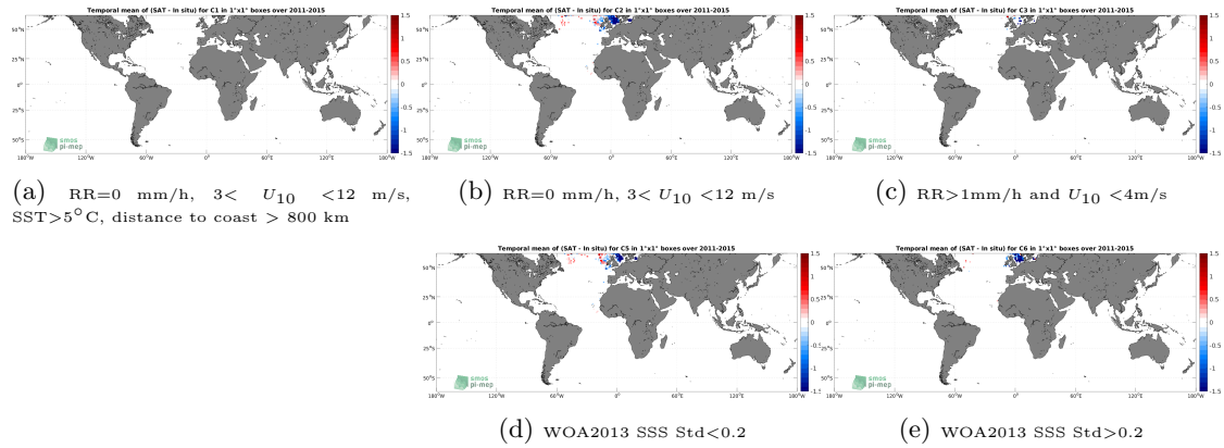
Figure 12: Temporal mean gridded over spatial boxes of size 1^\circ \times 1^\circ of \Delta SSS (Aquarius SSS L3 OR v5 - 7-Day running - Rain mask (NASA-GSFC) - ICES) for 5 different subdatasets corresponding to:RR=0 mm/h, 3 < U_{10} < 12 m/s, SST >5^\circ C, distance to coast > 800 km (a), RR=0 mm/h, 3 < U_{10} < 12 m/s (b), RR >1 mm/h and U_{10} < 4 m/s (c), WOA2013 SSS Std <0.2 (d), WOA2013 SSS Std >0.2 (e).
