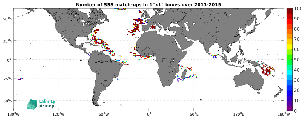
Figure 4: Number of SSS match-ups between Surface drifters SSS and the Aquarius SSS L3 OR v5 - 7-Day running - Rain mask (NASA-GSFC) SSS product for the SMOS coastal zone (<800km) 60N-60S Pi-MEP region over 1^\circ \times 1^\circ boxes and for the full satellite product period.
