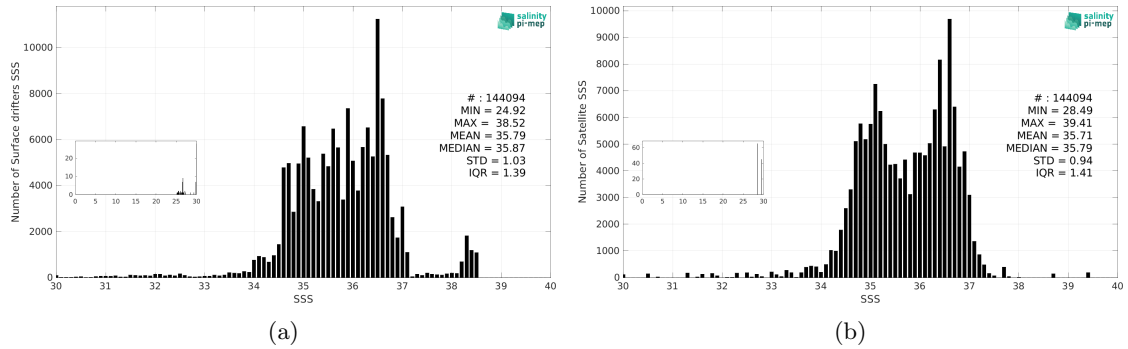
Figure 3: Histograms of SSS from Surface drifters (a) and Aquarius SSS L3 OR v5 - 7-Day running - Rain mask (NASA-GSFC) (b) considering all match-up pairs per bins of 0.1 over the SMOS coastal zone (<800km) 60N-60S Pi-MEP region and for the full satellite product period.
