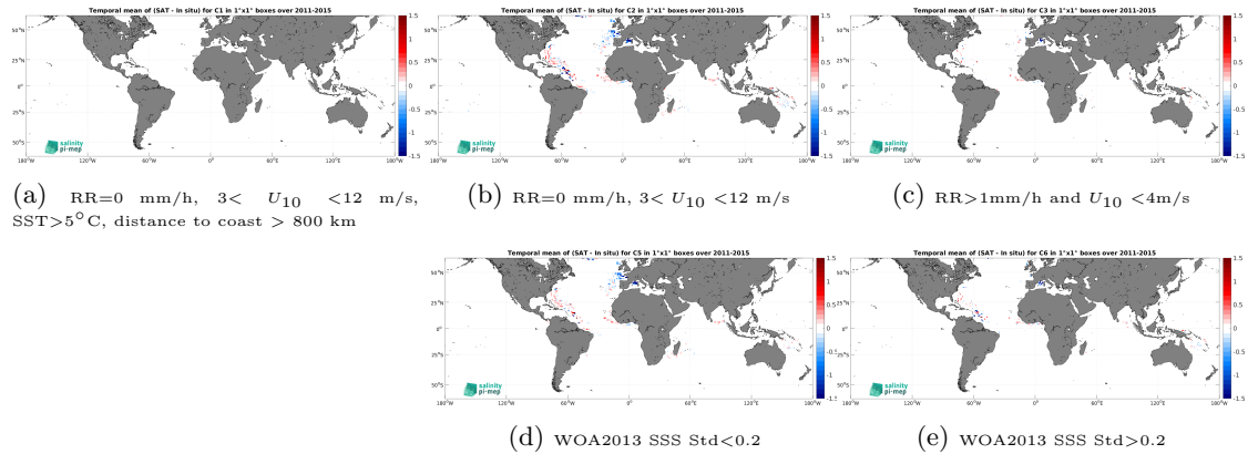
Figure 13: Temporal mean gridded over spatial boxes of size 1^\circ \times 1^\circ of \Delta SSS (Aquarius SSS L3 OR v5 - 7-Day running - Rain mask (NASA-GSFC) - Surface drifters) for 5 different subdatasets corresponding to:RR=0 mm/h, 3 < U_{10} < 12 m/s, SST >5^\circ\text{C} , distance to coast > 800 km (a), RR=0 mm/h, 3 < U_{10} < 12 m/s (b), RR >1 mm/h and U_{10} < 4 m/s (c), WOA2013 SSS Std <0.2 (d), WOA2013 SSS Std >0.2 (e).
