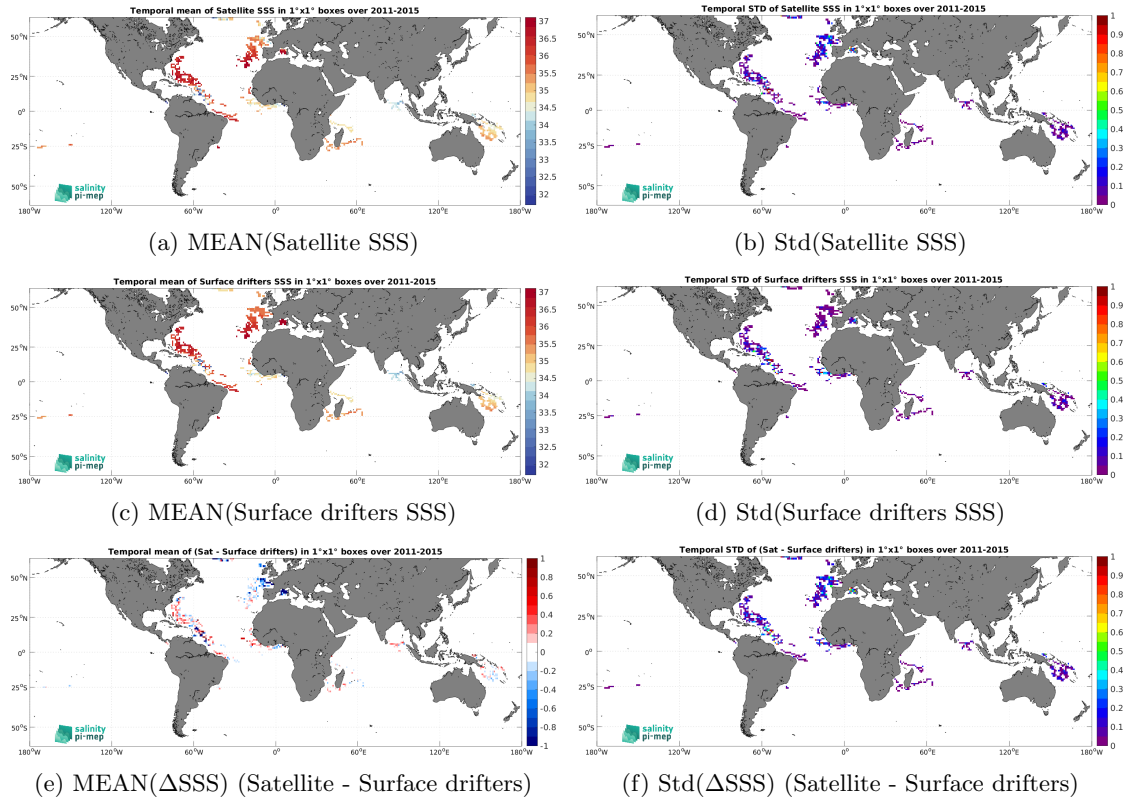
Figure 6: Temporal mean (left) and Std (right) of SSS from Aquarius SSS L3 OR v5 - 7-Day running - Rain mask (NASA-GSFC) (top), Surface drifters (middle), and of \Delta SSS (Satellite - Surface drifters). Only match-up pairs are used to generate these maps.
