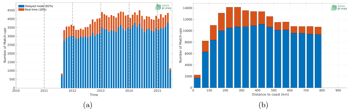
Figure 1: Number of match-ups between Argo and Aquarius SSS L3 OR v5 - 7-Day running - Rain mask (NASA-GSFC) SSS as a function of time (a) and as function of the distance to coast (b) over the SMOS coastal zone (<800km) 60N-60S Pi-MEP region and for the full satellite product period.
