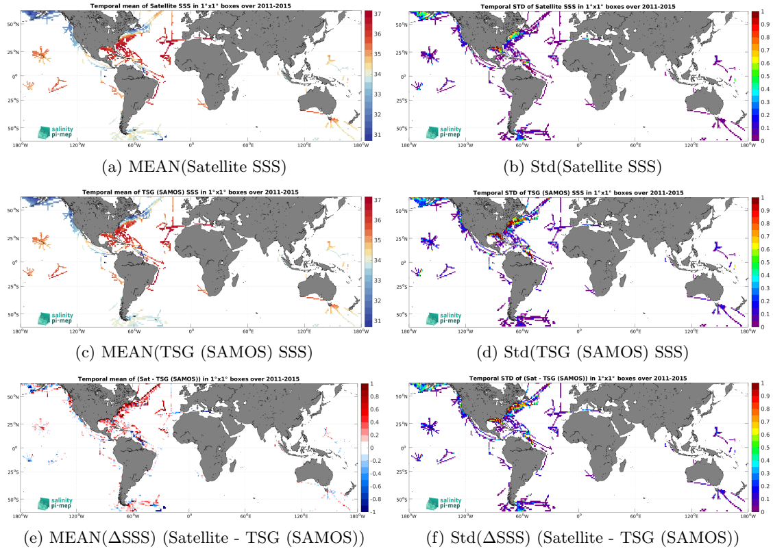
Figure 7: Temporal mean (left) and Std (right) of SSS from Aquarius SSS L3 OR v5 - Monthly (NASA-GSFC) (top), TSG (SAMOS) (middle), and of \Delta SSS (Satellite - TSG (SAMOS)). Only match-up pairs are used to generate these maps.
