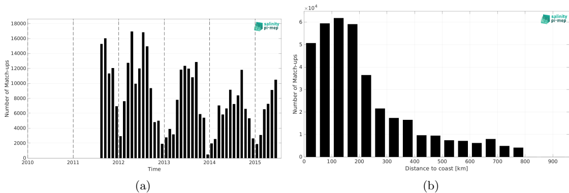
Figure 2: Number of match-ups between TSG (SAMOS) and Aquarius SSS L3 OR v5 - Monthly (NASA-GSFC) SSS as a function of time (a) and as function of the distance to coast (b) over the SMOS coastal zone (<800km) 60N-60S Pi-MEP region and for the full satellite product period.
