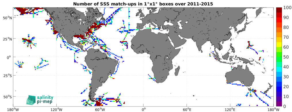
Figure 5: Number of SSS match-ups between TSG (SAMOS) SSS and the Aquarius SSS L3 OR v5 - Monthly (NASA-GSFC) SSS product for the SMOS coastal zone (<800km) 60N-60S Pi-MEP region over 1^\circ \times 1^\circ boxes and for the full satellite product period.
