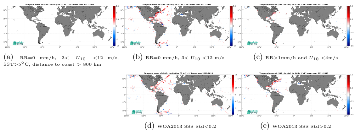
Figure 14: Temporal mean gridded over spatial boxes of size 1^\circ \times 1^\circ of \Delta SSS (Aquarius SSS L3 OR v5 - Monthly (NASA-GSFC) - TSG (SAMOS)) for 5 different subdatasets corresponding to: RR=0 mm/h, 3 < U_{10} < 12 m/s, SST > 5^\circ\text{C} , distance to coast > 800 km (a), RR=0 mm/h, 3 < U_{10} < 12 m/s (b), RR > 1 mm/h and U_{10} < 4 m/s (c), WOA2013 SSS Std < 0.2 (d), WOA2013 SSS Std > 0.2 (e).
