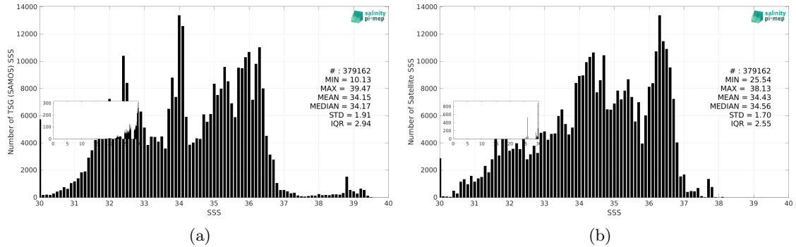
Figure 3: Histograms of SSS from TSG (SAMOS) (a) and Aquarius SSS L3 OR v5 - Monthly (NASA-GSFC) (b) considering all match-up pairs per bins of 0.1 over the SMOS coastal zone (<800km) 60N-60S Pi-MEP region and for the full satellite product period.
