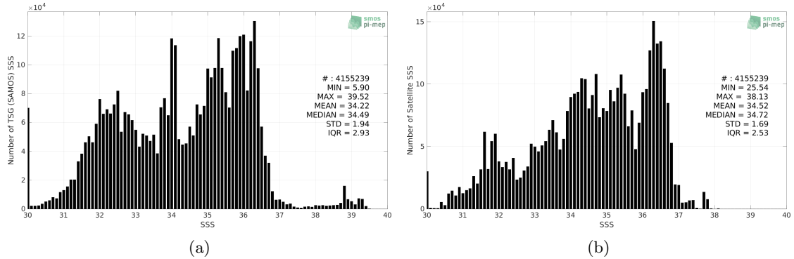
Figure 2: Histograms of SSS from TSG (SAMOS) (a) and Aquarius SSS L3 OR v5 - Monthly (NASA-GSFC) (b) considering all match-up pairs per bins of 0.1 over the SMOS coastal zone (<800km) 60N-60S Pi-MEP region and for the full satellite product period.
