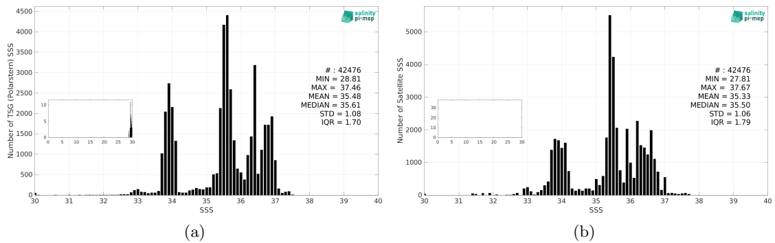
Figure 3: Histograms of SSS from TSG (Polarstern) (a) and Aquarius SSS L3 OR v5 - Monthly (NASA-GSFC) (b) considering all match-up pairs per bins of 0.1 over the SMOS coastal zone (<800km) 60N-60S Pi-MEP region and for the full satellite product period.
