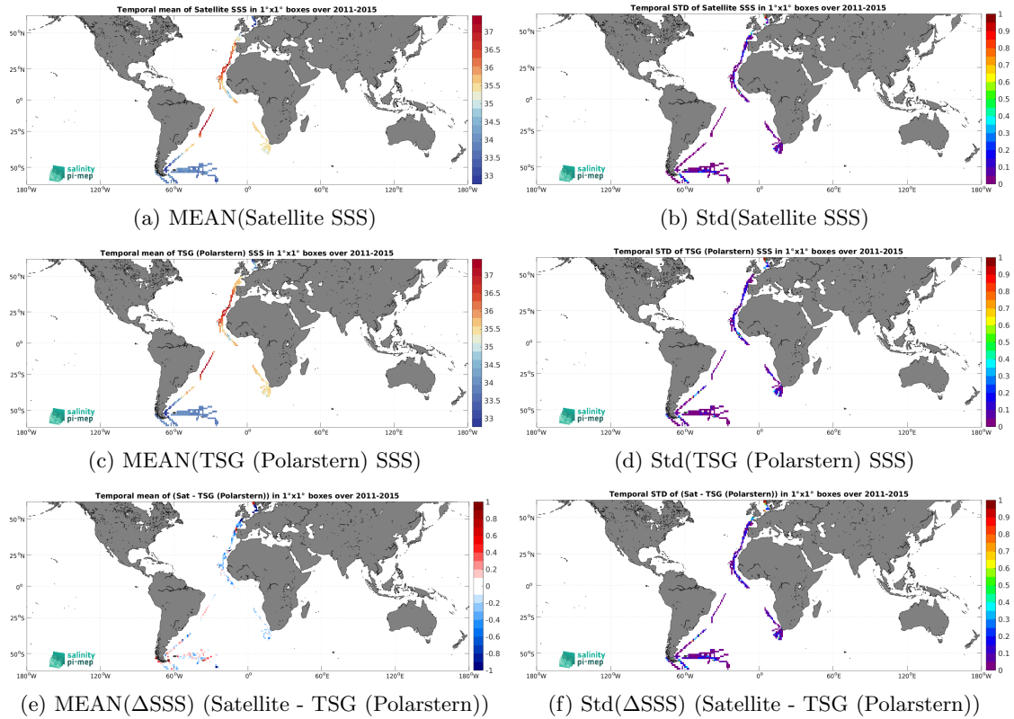
Figure 7: Temporal mean (left) and Std (right) of SSS from Aquarius SSS L3 OR v5 - Monthly (NASA-GSFC) (top), TSG (Polarstern) (middle), and of \Delta SSS (Satellite - TSG (Polarstern)). Only match-up pairs are used to generate these maps.
