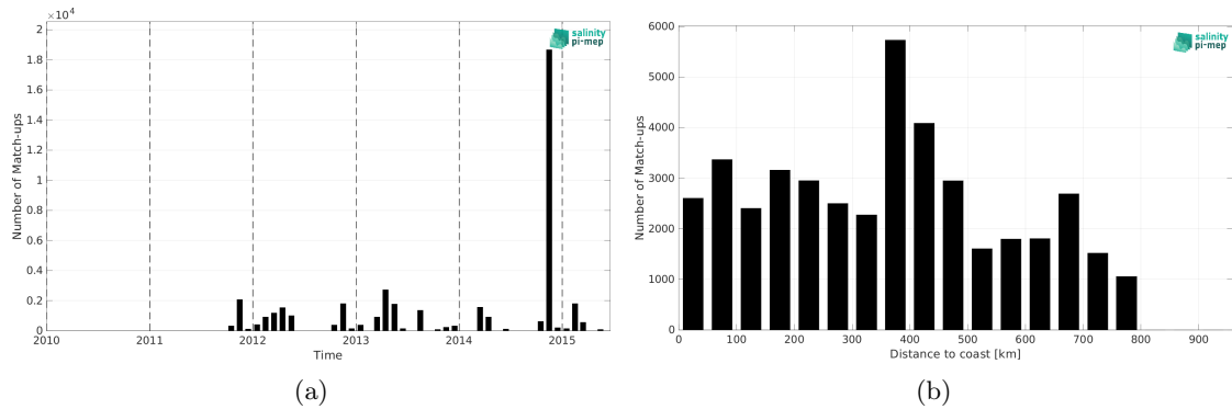
Figure 2: Number of match-ups between TSG (Polarstern) and Aquarius SSS L3 OR v5 - Monthly (NASA-GSFC) SSS as a function of time (a) and as function of the distance to coast (b) over the SMOS coastal zone (<800km) 60N-60S Pi-MEP region and for the full satellite product period.
