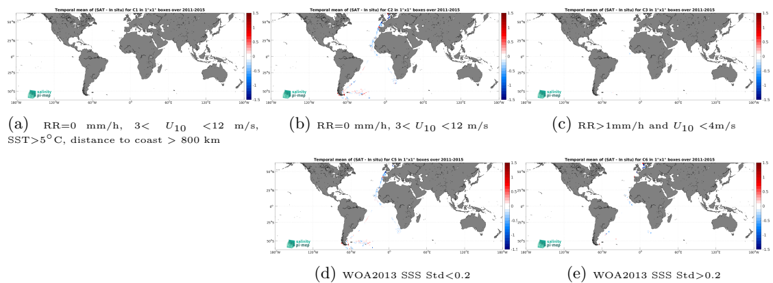
Figure 14: Temporal mean gridded over spatial boxes of size 1^\circ \times 1^\circ of \Delta SSS (Aquarius SSS L3 OR v5 - Monthly (NASA-GSFC) - TSG (Polarstern)) for 5 different subdatasets corresponding to: RR=0 mm/h, 3 < U_{10} < 12 m/s, SST > 5^\circ\text{C} , distance to coast > 800 km (a), RR=0 mm/h, 3 < U_{10} < 12 m/s (b), RR > 1 mm/h and U_{10} < 4 m/s (c), WOA2013 SSS Std < 0.2 (d), WOA2013 SSS Std > 0.2 (e).
