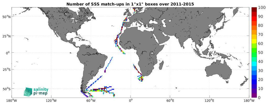
Figure 5: Number of SSS match-ups between TSG (Polarstern) SSS and the Aquarius SSS L3 OR v5 - Monthly (NASA-GSFC) SSS product for the SMOS coastal zone (<800km) 60N-60S Pi-MEP region over 1^\circ \times 1^\circ boxes and for the full satellite product period.
