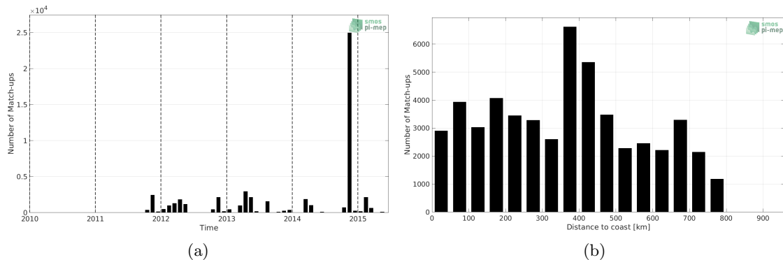
Figure 1: Number of match-ups between TSG (Polarstern) and Aquarius SSS L3 OR v5 - Monthly (NASA-GSFC) SSS as a function of time (a) and as function of the distance to coast (b) over the SMOS coastal zone (<800km) 60N-60S Pi-MEP region and for the full satellite product period.
