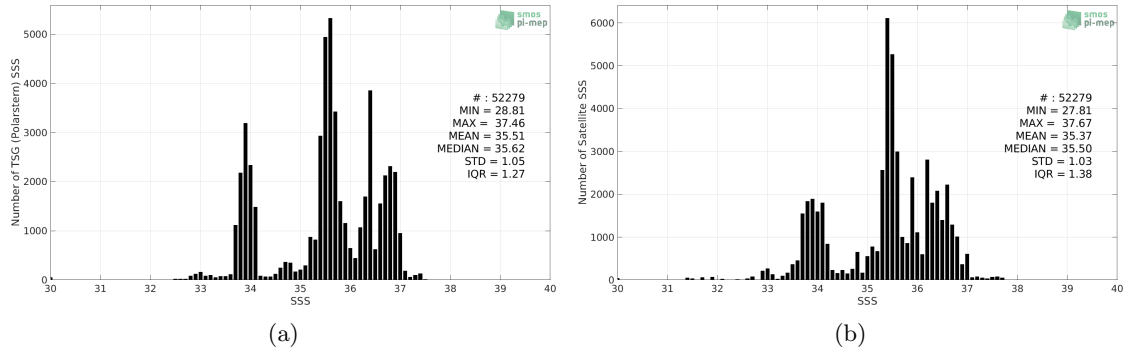
Figure 2: Histograms of SSS from TSG (Polarstern) (a) and Aquarius SSS L3 OR v5 - Monthly (NASA-GSFC) (b) considering all match-up pairs per bins of 0.1 over the SMOS coastal zone (<800km) 60N-60S Pi-MEP region and for the full satellite product period.
