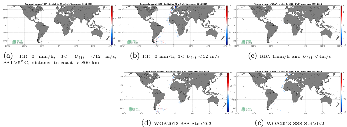
Figure 12: Temporal mean gridded over spatial boxes of size 1^\circ \times 1^\circ of \Delta\text{SSS} (Aquarius SSS L3 OR v5 - Monthly (NASA-GSFC) - TSG (Polarstern)) for 5 different subdatasets corresponding to:RR=0 mm/h, 3 < U_{10} < 12 m/s, SST >5^\circ\text{C} , distance to coast > 800 km (a), RR=0 mm/h, 3 < U_{10} < 12 m/s (b), RR >1 mm/h and U_{10} < 4 m/s (c), WOA2013 SSS Std <0.2 (d), WOA2013 SSS Std >0.2 (e).
