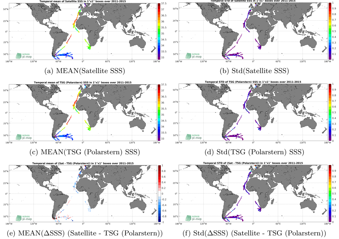
Figure 6: Temporal mean (left) and Std (right) of SSS from Aquarius SSS L3 OR v5 - Monthly (NASA-GSFC) (top), TSG (Polarstern) (middle), and of \Delta SSS (Satellite - TSG (Polarstern)). Only match-up pairs are used to generate these maps.
