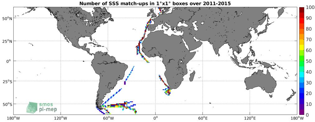
Figure 4: Number of SSS match-ups between TSG (Polarstern) SSS and the Aquarius SSS L3 OR v5 - Monthly (NASA-GSFC) SSS product for the SMOS coastal zone (<800km) 60N-60S Pi-MEP region over 1^\circ \times 1^\circ boxes and for the full satellite product period.
