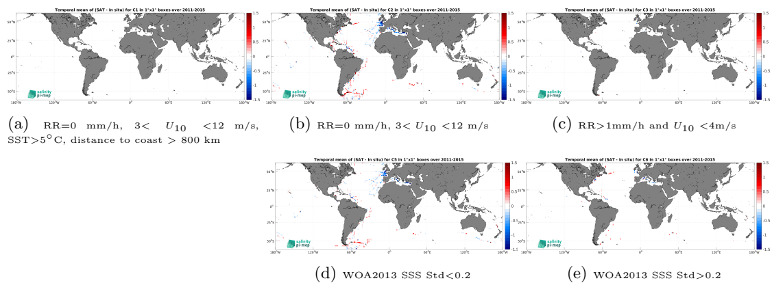
Figure 14: Temporal mean gridded over spatial boxes of size 1^\circ \times 1^\circ of \Delta\text{SSS} (Aquarius SSS L3 OR v5 - Monthly (NASA-GSFC) - TSG (GOSUD-Sailing-ship)) for 5 different subdatasets corresponding to: RR=0 mm/h, 3 < U_{10} < 12 m/s, SST > 5°C, distance to coast > 800 km (a), RR=0 mm/h, 3 < U_{10} < 12 m/s (b), RR > 1mm/h and U_{10} < 4 m/s (c), WOA2013 SSS Std < 0.2 (d), WOA2013 SSS Std > 0.2 (e).
