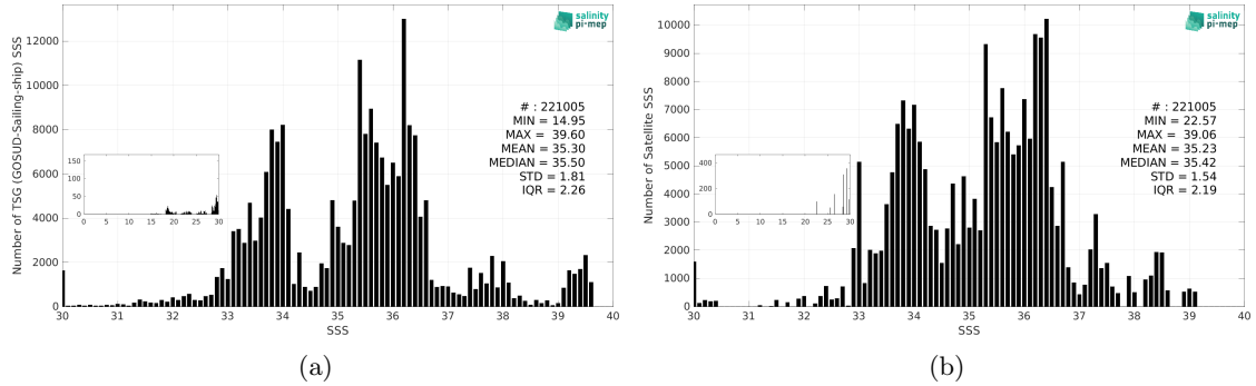
Figure 3: Histograms of SSS from TSG (GOSUD-Sailing-ship) (a) and Aquarius SSS L3 OR v5 - Monthly (NASA-GSFC) (b) considering all match-up pairs per bins of 0.1 over the SMOS coastal zone (<800km) 60N-60S Pi-MEP region and for the full satellite product period.
