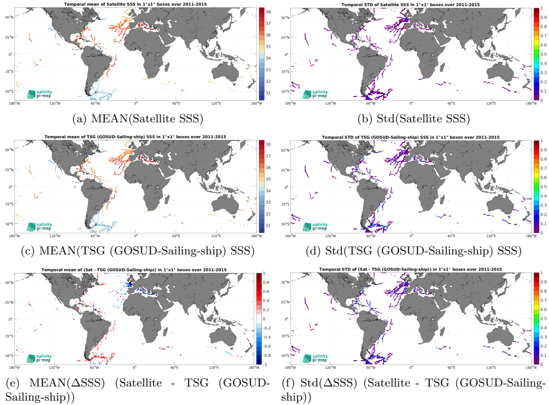
Figure 7: Temporal mean (left) and Std (right) of SSS from Aquarius SSS L3 OR v5 - Monthly (NASA-GSFC) (top), TSG (GOSUD-Sailing-ship) (middle), and of \Delta SSS (Satellite - TSG (GOSUD-Sailing-ship)). Only match-up pairs are used to generate these maps.
