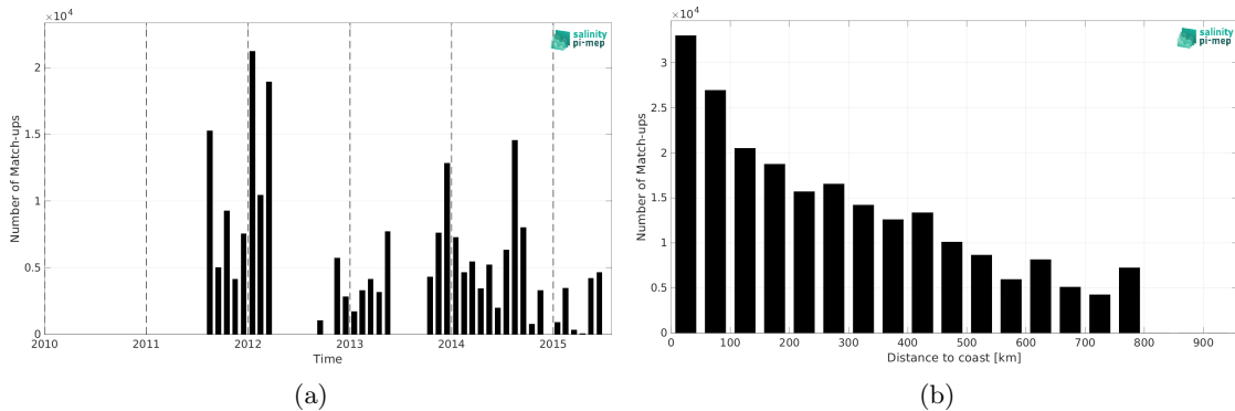
Figure 2: Number of match-ups between TSG (GOSUD-Sailing-ship) and Aquarius SSS L3 OR v5 - Monthly (NASA-GSFC) SSS as a function of time (a) and as function of the distance to coast (b) over the SMOS coastal zone (<800km) 60N-60S Pi-MEP region and for the full satellite product period.
