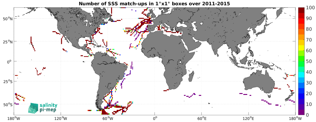
Figure 5: Number of SSS match-ups between TSG (GOSUD-Sailing-ship) SSS and the Aquarius SSS L3 OR v5 - Monthly (NASA-GSFC) SSS product for the SMOS coastal zone (<800km) 60N-60S Pi-MEP region over 1^\circ \times 1^\circ boxes and for the full satellite product period.
