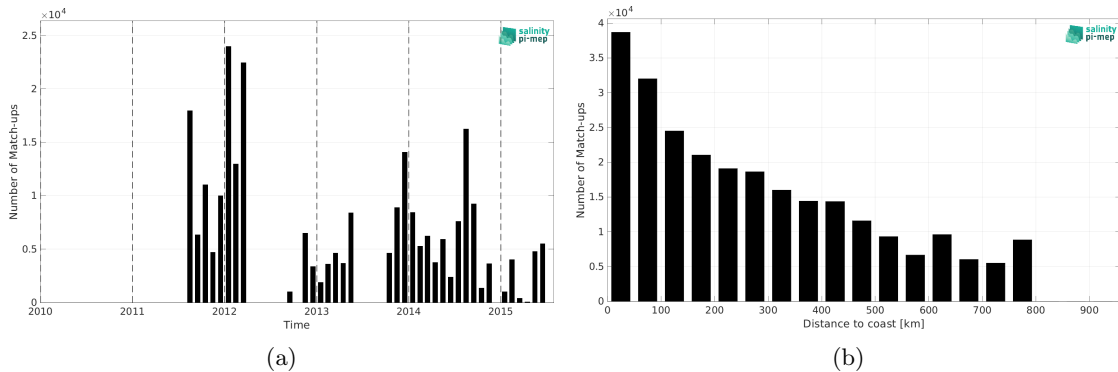
Figure 1: Number of match-ups between TSG (GOSUD-Sailing-ship) and Aquarius SSS L3 OR v5 - Monthly (NASA-GSFC) SSS as a function of time (a) and as function of the distance to coast (b) over the SMOS coastal zone (<800km) 60N-60S Pi-MEP region and for the full satellite product period.
