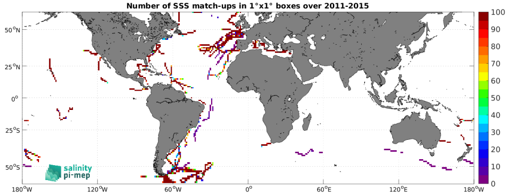
Figure 4: Number of SSS match-ups between TSG (GOSUD-Sailing-ship) SSS and the Aquarius SSS L3 OR v5 - Monthly (NASA-GSFC) SSS product for the SMOS coastal zone (<800km) 60N-60S Pi-MEP region over 1^\circ \times 1^\circ boxes and for the full satellite product period.
