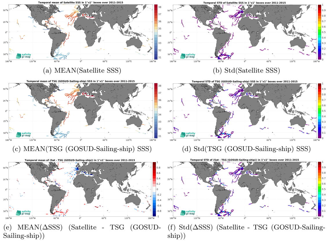
Figure 6: Temporal mean (left) and Std (right) of SSS from Aquarius SSS L3 OR v5 - Monthly (NASA-GSFC) (top), TSG (GOSUD-Sailing-ship) (middle), and of \Delta SSS (Satellite - TSG (GOSUD-Sailing-ship)). Only match-up pairs are used to generate these maps.
