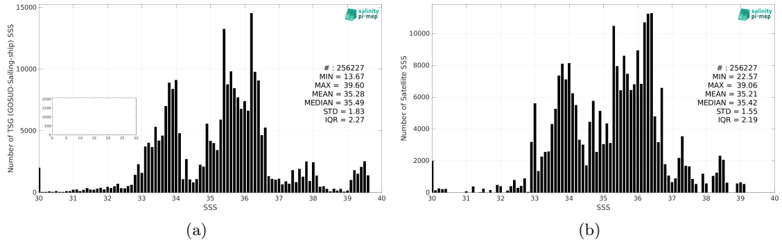
Figure 2: Histograms of SSS from TSG (GOSUD-Sailing-ship) (a) and Aquarius SSS L3 OR v5 - Monthly (NASA-GSFC) (b) considering all match-up pairs per bins of 0.1 over the SMOS coastal zone (<800km) 60N-60S Pi-MEP region and for the full satellite product period.
