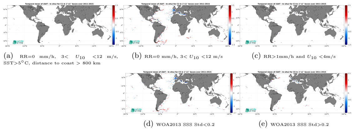
Figure 12: Temporal mean gridded over spatial boxes of size 1^\circ \times 1^\circ of \Delta\text{SSS} (Aquarius SSS L3 OR v5 - Monthly (NASA-GSFC) - TSG (GOSUD-Sailing-ship)) for 5 different subdatasets corresponding to: RR=0 mm/h, 3 < U_{10} < 12 m/s, SST > 5°C, distance to coast > 800 km (a), RR=0 mm/h, 3 < U_{10} < 12 m/s (b), RR > 1mm/h and U_{10} < 4 m/s (c), WOA2013 SSS Std < 0.2 (d), WOA2013 SSS Std > 0.2 (e).
