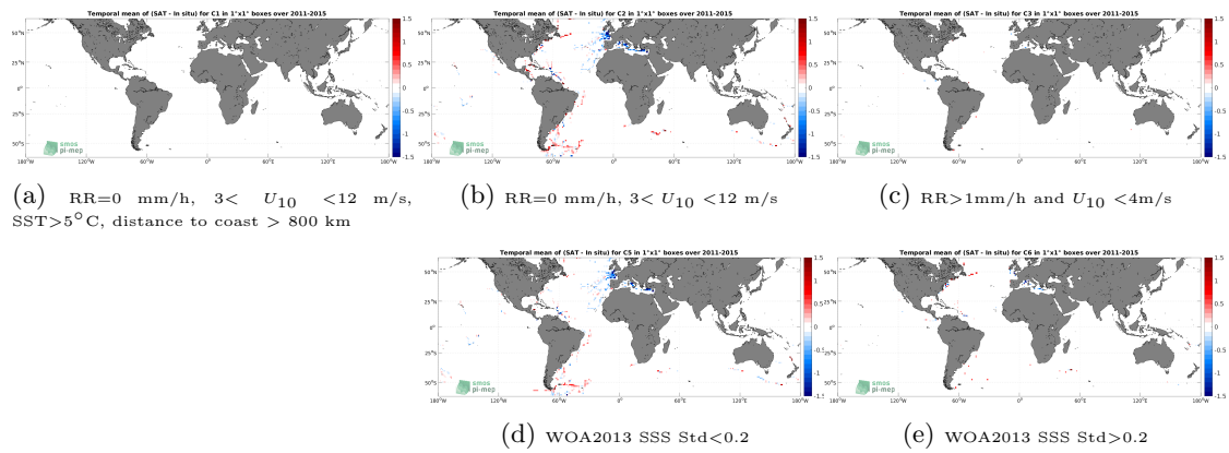
Figure 12: Temporal mean gridded over spatial boxes of size 1^\circ \times 1^\circ of \Delta SSS (Aquarius SSS L3 OR v5 - Monthly (NASA-GSFC) - TSG (GOSUD-Sailing-ship)) for 5 different subdatasets corresponding to: RR=0 mm/h, 3 < U_{10} < 12 m/s, SST > 5^\circ\text{C} , distance to coast > 800 km (a), RR=0 mm/h, 3 < U_{10} < 12 m/s (b), RR > 1 mm/h and U_{10} < 4 m/s (c), WOA2013 SSS Std < 0.2 (d), WOA2013 SSS Std > 0.2 (e).
