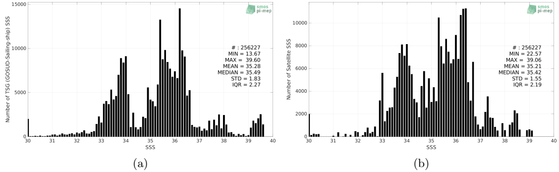
Figure 2: Histograms of SSS from TSG (GOSUD-Sailing-ship) (a) and Aquarius SSS L3 OR v5 - Monthly (NASA-GSFC) (b) considering all match-up pairs per bins of 0.1 over the SMOS coastal zone (<800km) 60N-60S Pi-MEP region and for the full satellite product period.
