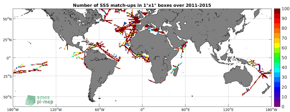
Figure 4: Number of SSS match-ups between TSG-GOSUD-Research-vessel SSS and the Aquarius-L3-OR-V5-MONTHLY-1DEG SSS product for the SMOS coastal zone ( \pm 800\text{km} ) 60N-60S Pi-MEP region over 1^\circ \times 1^\circ boxes and for the full satellite product period.
