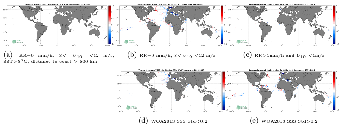
Figure 12: Temporal mean gridded over spatial boxes of size 1^\circ \times 1^\circ of \Delta\text{SSS} (Aquarius-L3-OR-V5-MONTHLY-1DEG - TSG-GOSUD-Research-vessel) for 5 different subdatasets corresponding to:RR=0 mm/h, 3 < U_{10} < 12 m/s, SST>5°C, distance to coast > 800 km (a), RR=0 mm/h, 3 < U_{10} < 12 m/s (b), RR>1mm/h and U_{10} < 4 m/s (c), WOA2013 SSS Std<0.2 (d), WOA2013 SSS Std>0.2 (e).
