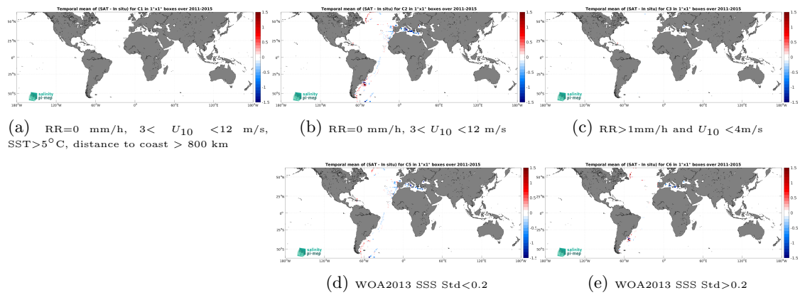
Figure 14: Temporal mean gridded over spatial boxes of size 1^\circ \times 1^\circ of \Delta\text{SSS} (Aquarius SSS L3 OR v5 - Monthly (NASA-GSFC) - TSG (CSIC-UTM)) for 5 different subdatasets corresponding to: RR=0 mm/h, 3 < U_{10} < 12 m/s, SST > 5°C, distance to coast > 800 km (a), RR=0 mm/h, 3 < U_{10} < 12 m/s (b), RR > 1mm/h and U_{10} < 4 m/s (c), WOA2013 SSS Std < 0.2 (d), WOA2013 SSS Std > 0.2 (e).
