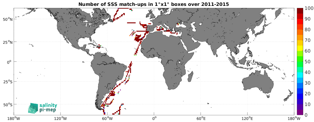
Figure 5: Number of SSS match-ups between TSG (CSIC-UTM) SSS and the Aquarius SSS L3 OR v5 - Monthly (NASA-GSFC) SSS product for the SMOS coastal zone (<800km) 60N-60S Pi-MEP region over 1^{\circ} \times 1^{\circ} boxes and for the full satellite product period.
