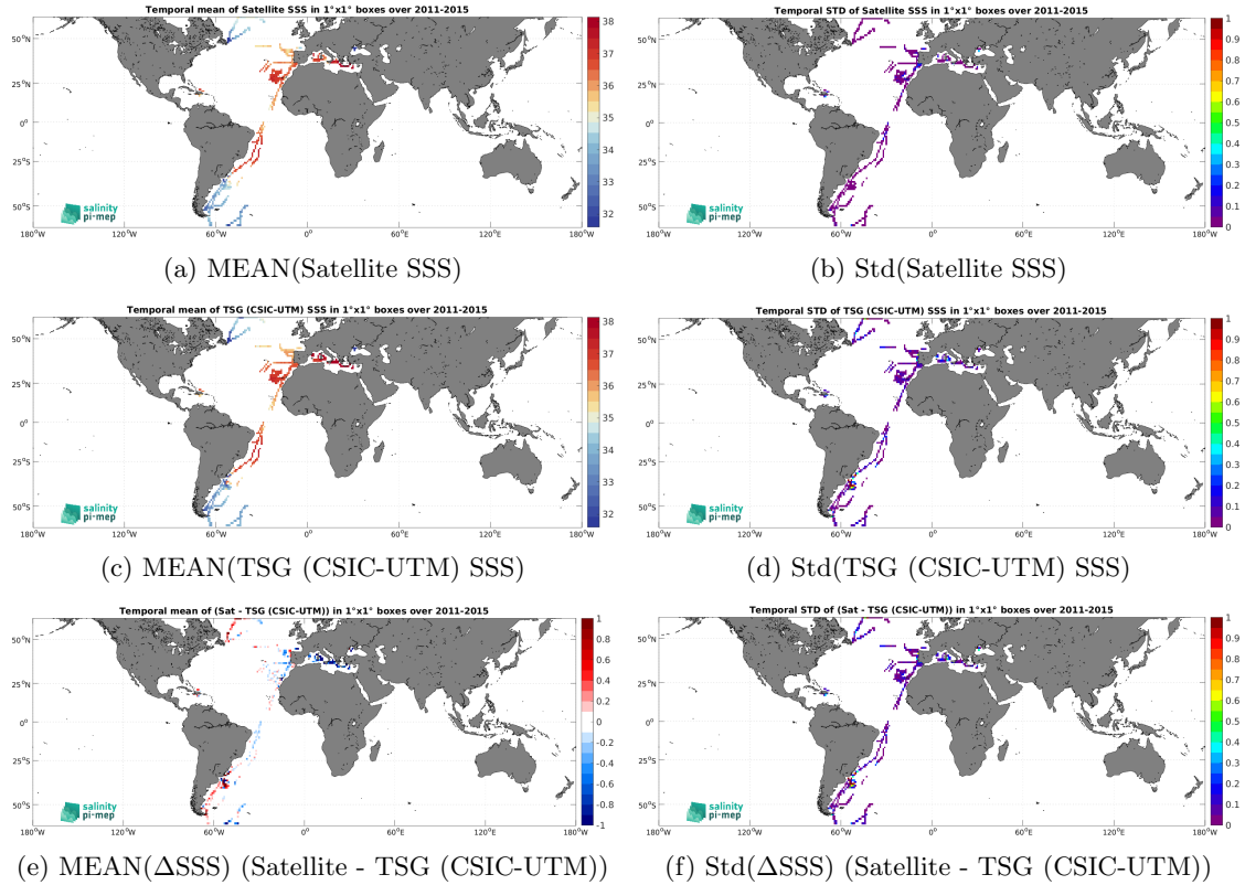
Figure 7: Temporal mean (left) and Std (right) of SSS from Aquarius SSS L3 OR v5 - Monthly (NASA-GSFC) (top), TSG (CSIC-UTM) (middle), and of \Delta SSS (Satellite - TSG (CSIC-UTM)). Only match-up pairs are used to generate these maps.
