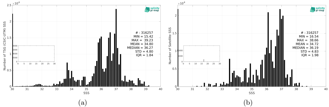
Figure 3: Histograms of SSS from TSG (CSIC-UTM) (a) and Aquarius SSS L3 OR v5 - Monthly (NASA-GSFC) (b) considering all match-up pairs per bins of 0.1 over the SMOS coastal zone (<800km) 60N-60S Pi-MEP region and for the full satellite product period.
