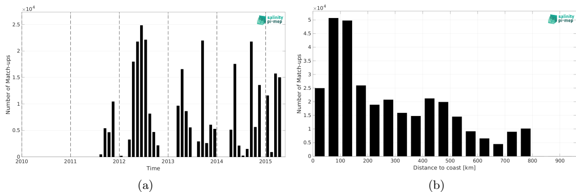
Figure 2: Number of match-ups between TSG (CSIC-UTM) and Aquarius SSS L3 OR v5 - Monthly (NASA-GSFC) SSS as a function of time (a) and as function of the distance to coast (b) over the SMOS coastal zone (<800km) 60N-60S Pi-MEP region and for the full satellite product period.
