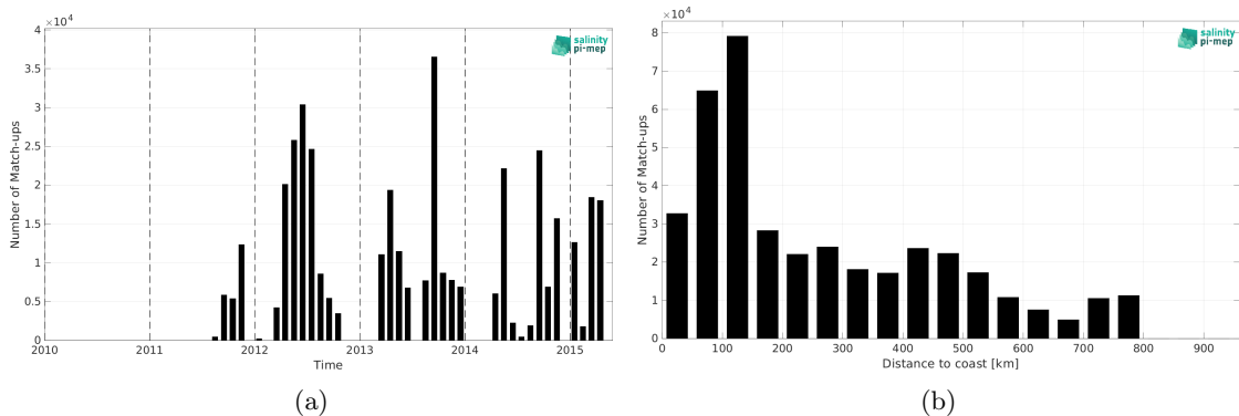
Figure 1: Number of match-ups between TSG (CSIC-UTM) and Aquarius SSS L3 OR v5 - Monthly (NASA-GSFC) SSS as a function of time (a) and as function of the distance to coast (b) over the SMOS coastal zone (<800km) 60N-60S Pi-MEP region and for the full satellite product period.
