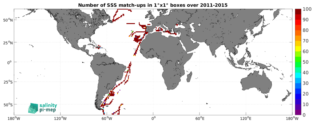
Figure 4: Number of SSS match-ups between TSG (CSIC-UTM) SSS and the Aquarius SSS L3 OR v5 - Monthly (NASA-GSFC) SSS product for the SMOS coastal zone (<800km) 60N-60S Pi-MEP region over 1^{\circ} \times 1^{\circ} boxes and for the full satellite product period.
