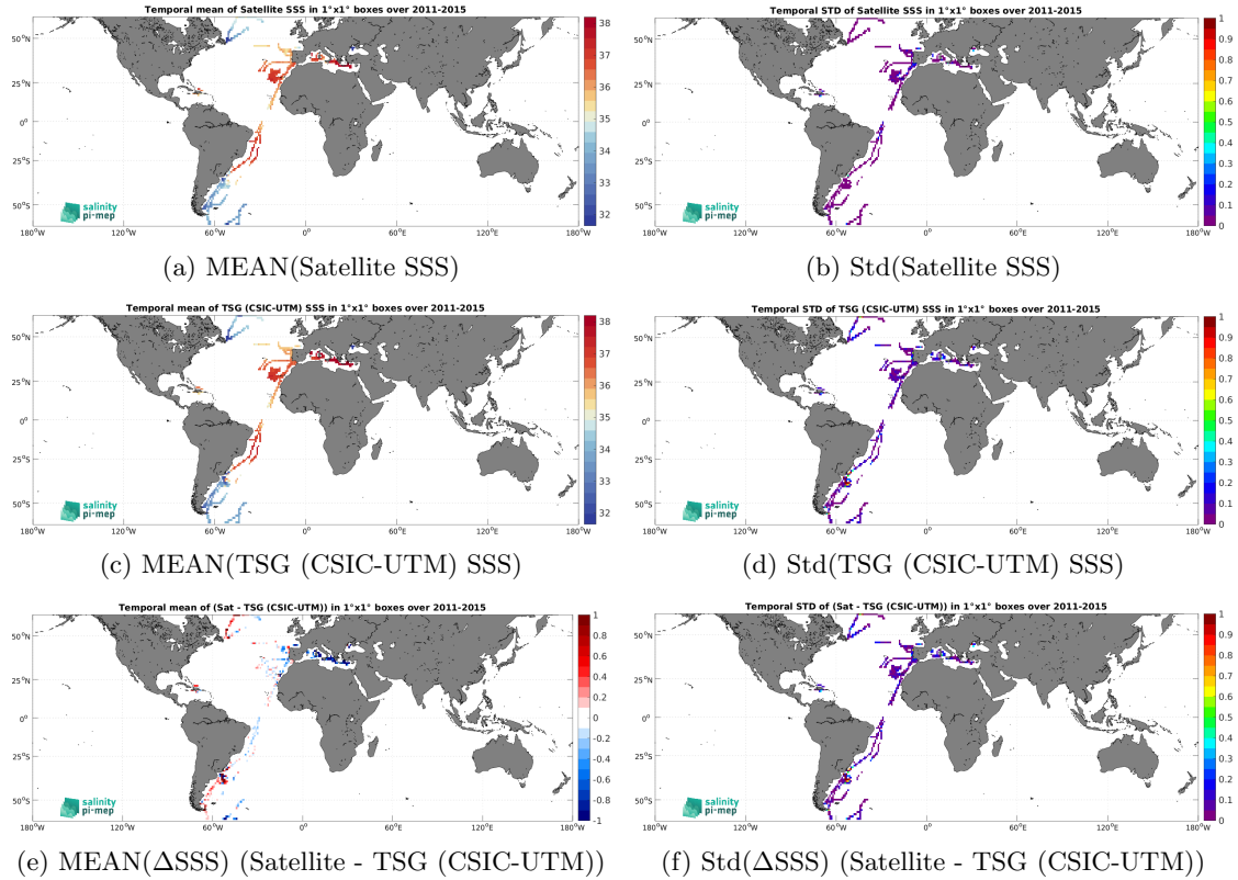
Figure 6: Temporal mean (left) and Std (right) of SSS from Aquarius SSS L3 OR v5 - Monthly (NASA-GSFC) (top), TSG (CSIC-UTM) (middle), and of \Delta SSS (Satellite - TSG (CSIC-UTM)). Only match-up pairs are used to generate these maps.
