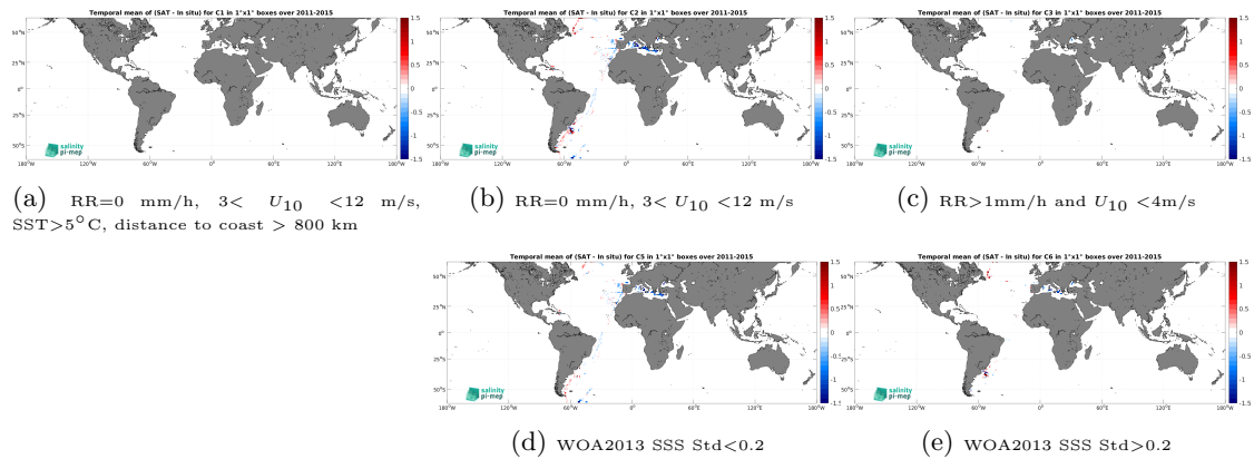
Figure 12: Temporal mean gridded over spatial boxes of size 1^\circ \times 1^\circ of \Delta SSS (Aquarius SSS L3 OR v5 - Monthly (NASA-GSFC) - TSG (CSIC-UTM)) for 5 different subdatasets corresponding to:RR=0 mm/h, 3 < U_{10} < 12 m/s, SST >5^\circ\text{C} , distance to coast > 800 km (a), RR=0 mm/h, 3 < U_{10} < 12 m/s (b), RR >1 mm/h and U_{10} < 4 m/s (c), WOA2013 SSS Std <0.2 (d), WOA2013 SSS Std >0.2 (e).
