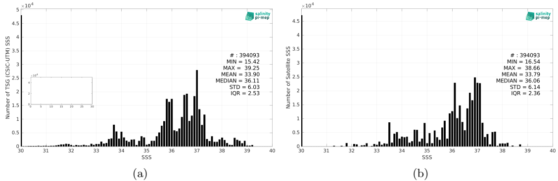
Figure 2: Histograms of SSS from TSG (CSIC-UTM) (a) and Aquarius SSS L3 OR v5 - Monthly (NASA-GSFC) (b) considering all match-up pairs per bins of 0.1 over the SMOS coastal zone (<800km) 60N-60S Pi-MEP region and for the full satellite product period.
