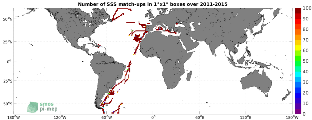
Figure 4: Number of SSS match-ups between TSG (CSIC-UTM) SSS and the Aquarius SSS L3 OR v5 - Monthly (NASA-GSFC) SSS product for the SMOS coastal zone (<800km) 60N-60S Pi-MEP region over 1^\circ \times 1^\circ boxes and for the full satellite product period.
