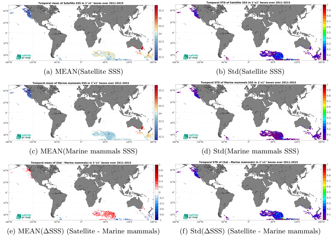
Figure 7: Temporal mean (left) and Std (right) of SSS from Aquarius SSS L3 OR v5 - Monthly (NASA-GSFC) (top), Marine mammals (middle), and of \Delta SSS (Satellite - Marine mammals). Only match-up pairs are used to generate these maps.
