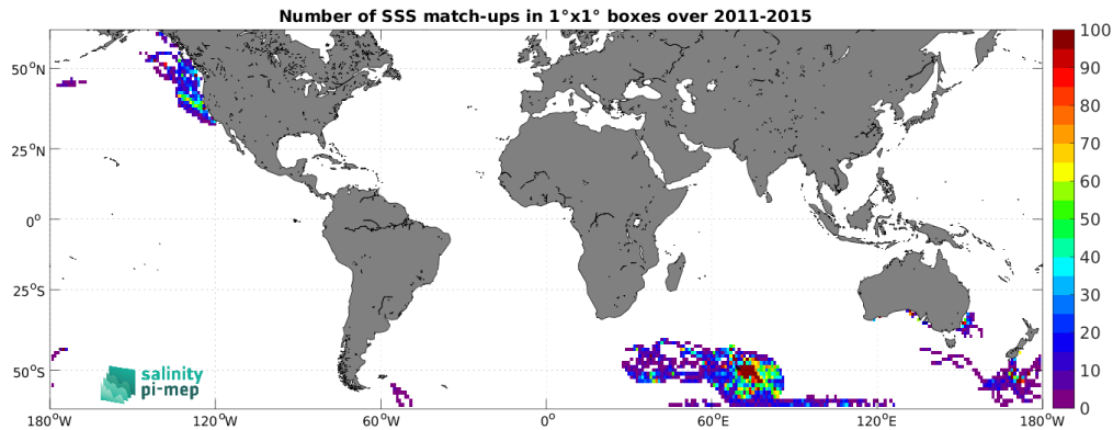
Figure 5: Number of SSS match-ups between Marine mammals SSS and the Aquarius SSS L3 OR v5 - Monthly (NASA-GSFC) SSS product for the SMOS coastal zone (<800km) 60N-60S Pi-MEP region over 1°x1° boxes and for the full satellite product period.
