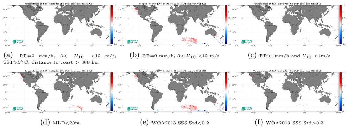
Figure 14: Temporal mean gridded over spatial boxes of size 1^\circ \times 1^\circ of \Delta SSS (Aquarius SSS L3 OR v5 - Monthly (NASA-GSFC) - Marine mammals) for 6 different subdatasets corresponding to:RR=0 mm/h, 3 < U_{10} < 12 m/s, SST >5^\circ C, distance to coast > 800 km (a), RR=0 mm/h, 3 < U_{10} < 12 m/s (b), RR >1 mm/h and U_{10} < 4 m/s (c),MLD <20 m (d),WOA2013 SSS Std <0.2 (e),WOA2013 SSS Std >0.2 (f).
