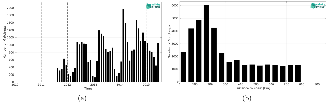
Figure 2: Number of match-ups between Marine mammals and Aquarius SSS L3 OR v5 - Monthly (NASA-GSFC) SSS as a function of time (a) and as function of the distance to coast (b) over the SMOS coastal zone (<800km) 60N-60S Pi-MEP region and for the full satellite product period.
