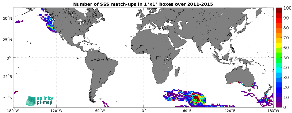
Figure 4: Number of SSS match-ups between Marine mammals SSS and the Aquarius SSS L3 OR v5 - Monthly (NASA-GSFC) SSS product for the SMOS coastal zone (<800km) 60N-60S Pi-MEP region over 1°x1° boxes and for the full satellite product period.
