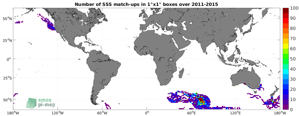
Figure 4: Number of SSS match-ups between Marine mammals SSS and the Aquarius SSS L3 OR v5 - Monthly (NASA-GSFC) SSS product for the SMOS coastal zone (<800km) 60N-60S Pi-MEP region over 1^\circ \times 1^\circ boxes and for the full satellite product period.
