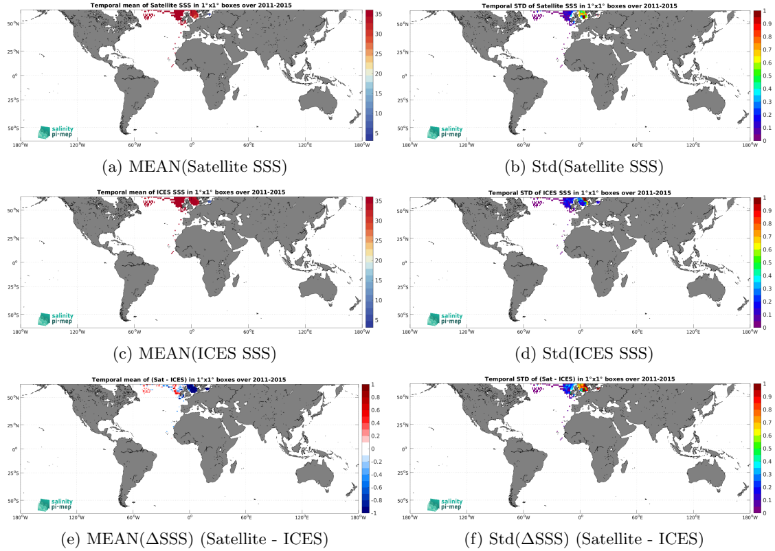
Figure 7: Temporal mean (left) and Std (right) of SSS from Aquarius SSS L3 OR v5 - Monthly (NASA-GSFC) (top), ICES (middle), and of \Delta SSS (Satellite - ICES). Only match-up pairs are used to generate these maps.
