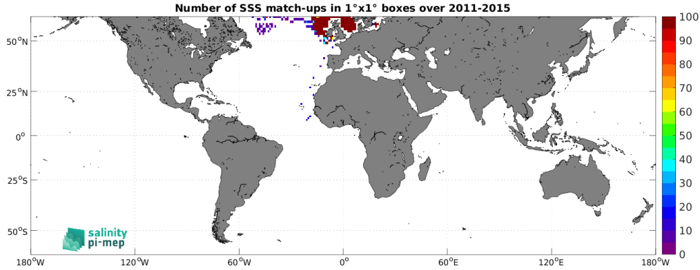
Figure 5: Number of SSS match-ups between ICES SSS and the Aquarius SSS L3 OR v5 - Monthly (NASA-GSFC) SSS product for the SMOS coastal zone (<800km) 60N-60S Pi-MEP region over 1^{\circ} \times 1^{\circ} boxes and for the full satellite product period.
