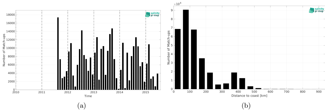
Figure 2: Number of match-ups between ICES and Aquarius SSS L3 OR v5 - Monthly (NASA-GSFC) SSS as a function of time (a) and as function of the distance to coast (b) over the SMOS coastal zone (<800km) 60N-60S Pi-MEP region and for the full satellite product period.
