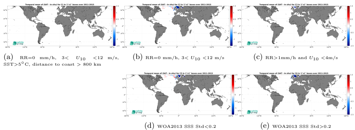
Figure 14: Temporal mean gridded over spatial boxes of size 1^\circ \times 1^\circ of \Delta SSS (Aquarius SSS L3 OR v5 - Monthly (NASA-GSFC) - ICES) for 5 different subdatasets corresponding to:RR=0 mm/h, 3 < U_{10} < 12 m/s, SST > 5^\circ\text{C} , distance to coast > 800 km (a), RR=0 mm/h, 3 < U_{10} < 12 m/s (b), RR > 1 mm/h and U_{10} < 4 m/s (c), WOA2013 SSS Std < 0.2 (d), WOA2013 SSS Std > 0.2 (e).
