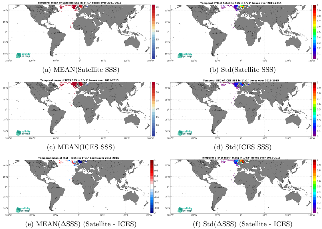
Figure 6: Temporal mean (left) and Std (right) of SSS from Aquarius SSS L3 OR v5 - Monthly (NASA-GSFC) (top), ICES (middle), and of \Delta SSS (Satellite - ICES). Only match-up pairs are used to generate these maps.
