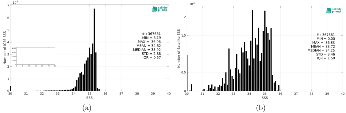
Figure 2: Histograms of SSS from ICES (a) and Aquarius SSS L3 OR v5 - Monthly (NASA-GSFC) (b) considering all match-up pairs per bins of 0.1 over the SMOS coastal zone (<800km) 60N-60S Pi-MEP region and for the full satellite product period.
