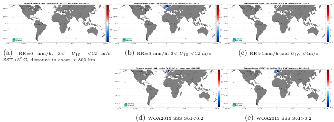
Figure 12: Temporal mean gridded over spatial boxes of size 1^\circ \times 1^\circ of \Delta SSS (Aquarius SSS L3 OR v5 - Monthly (NASA-GSFC) - ICES) for 5 different subdatasets corresponding to:RR=0 mm/h, 3 < U_{10} < 12 m/s, SST >5^\circ\text{C} , distance to coast > 800 km (a), RR=0 mm/h, 3 < U_{10} < 12 m/s (b), RR >1 mm/h and U_{10} < 4 m/s (c), WOA2013 SSS Std <0.2 (d), WOA2013 SSS Std >0.2 (e).
