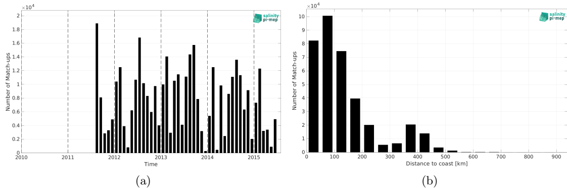
Figure 1: Number of match-ups between ICES and Aquarius SSS L3 OR v5 - Monthly (NASA-GSFC) SSS as a function of time (a) and as function of the distance to coast (b) over the SMOS coastal zone (<800km) 60N-60S Pi-MEP region and for the full satellite product period.
