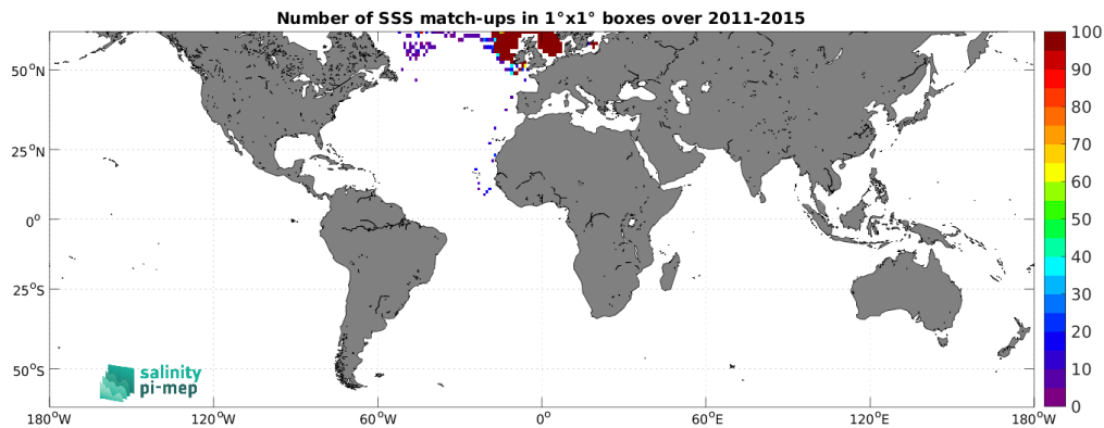
Figure 4: Number of SSS match-ups between ICES SSS and the Aquarius SSS L3 OR v5 - Monthly (NASA-GSFC) SSS product for the SMOS coastal zone (<800km) 60N-60S Pi-MEP region over 1^{\circ} \times 1^{\circ} boxes and for the full satellite product period.
