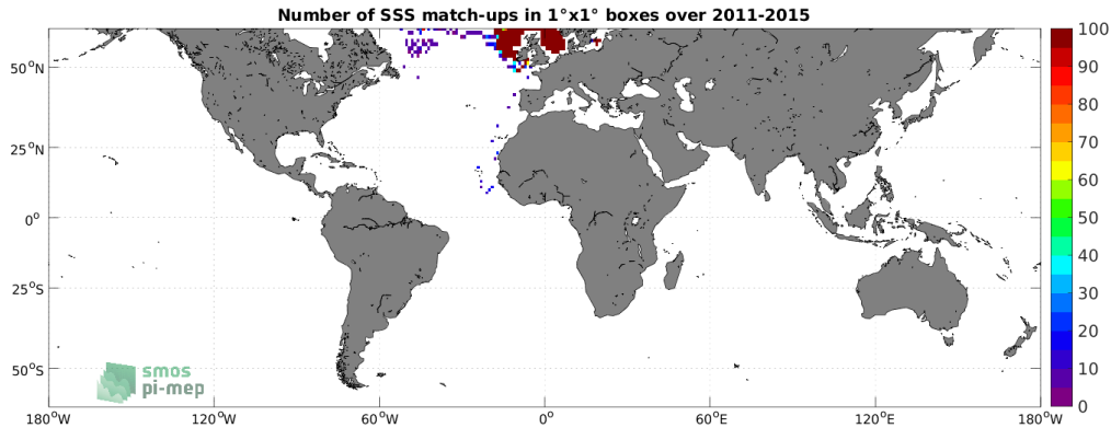
Figure 4: Number of SSS match-ups between ICES SSS and the Aquarius SSS L3 OR v5 - Monthly (NASA-GSFC) SSS product for the SMOS coastal zone (<800km) 60N-60S Pi-MEP region over 1^\circ \times 1^\circ boxes and for the full satellite product period.
