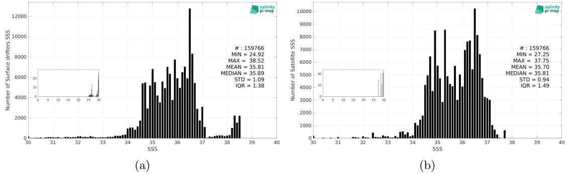
Figure 3: Histograms of SSS from Surface drifters (a) and Aquarius SSS L3 OR v5 - Monthly (NASA-GSFC) (b) considering all match-up pairs per bins of 0.1 over the SMOS coastal zone (<800km) 60N-60S Pi-MEP region and for the full satellite product period.
