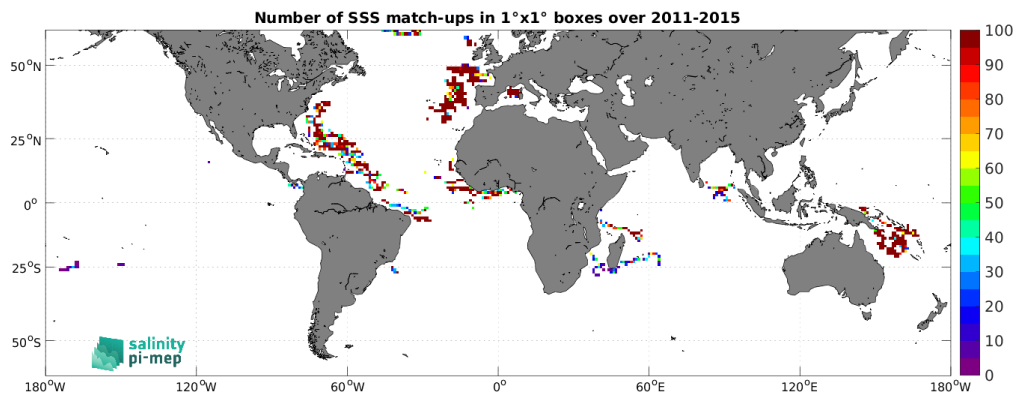
Figure 4: Number of SSS match-ups between Surface drifters SSS and the Aquarius SSS L3 OR v5 - Monthly (NASA-GSFC) SSS product for the SMOS coastal zone (<800km) 60N-60S Pi-MEP region over 1^\circ \times 1^\circ boxes and for the full satellite product period.
