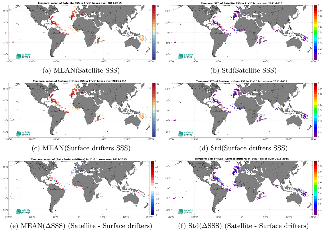
Figure 6: Temporal mean (left) and Std (right) of SSS from Aquarius SSS L3 OR v5 - Monthly (NASA-GSFC) (top), Surface drifters (middle), and of \Delta SSS (Satellite - Surface drifters). Only match-up pairs are used to generate these maps.
