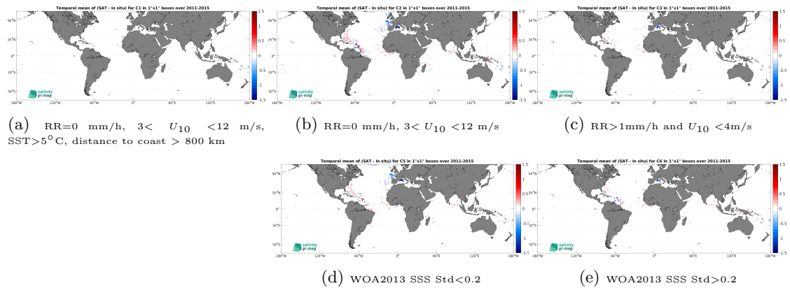
Figure 13: Temporal mean gridded over spatial boxes of size 1^\circ \times 1^\circ of \Delta SSS (Aquarius SSS L3 OR v5 - Monthly (NASA-GSFC) - Surface drifters) for 5 different subdatasets corresponding to:RR=0 mm/h, 3 < U_{10} < 12 m/s, SST >5^\circ\text{C} , distance to coast > 800 km (a), RR=0 mm/h, 3 < U_{10} < 12 m/s (b), RR >1 mm/h and U_{10} < 4 m/s (c), WOA2013 SSS Std <0.2 (d), WOA2013 SSS Std >0.2 (e).
