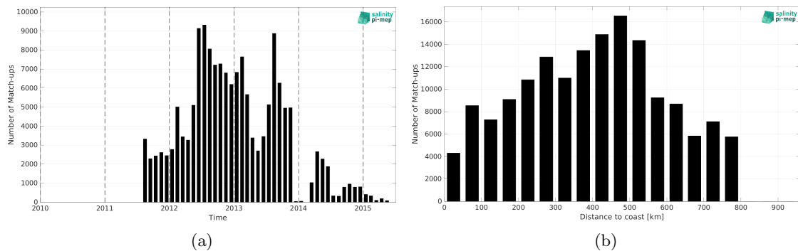
Figure 2: Number of match-ups between Surface drifters and Aquarius SSS L3 OR v5 - Monthly (NASA-GSFC) SSS as a function of time (a) and as function of the distance to coast (b) over the SMOS coastal zone ( < 800\text{km} ) 60N-60S Pi-MEP region and for the full satellite product period.
