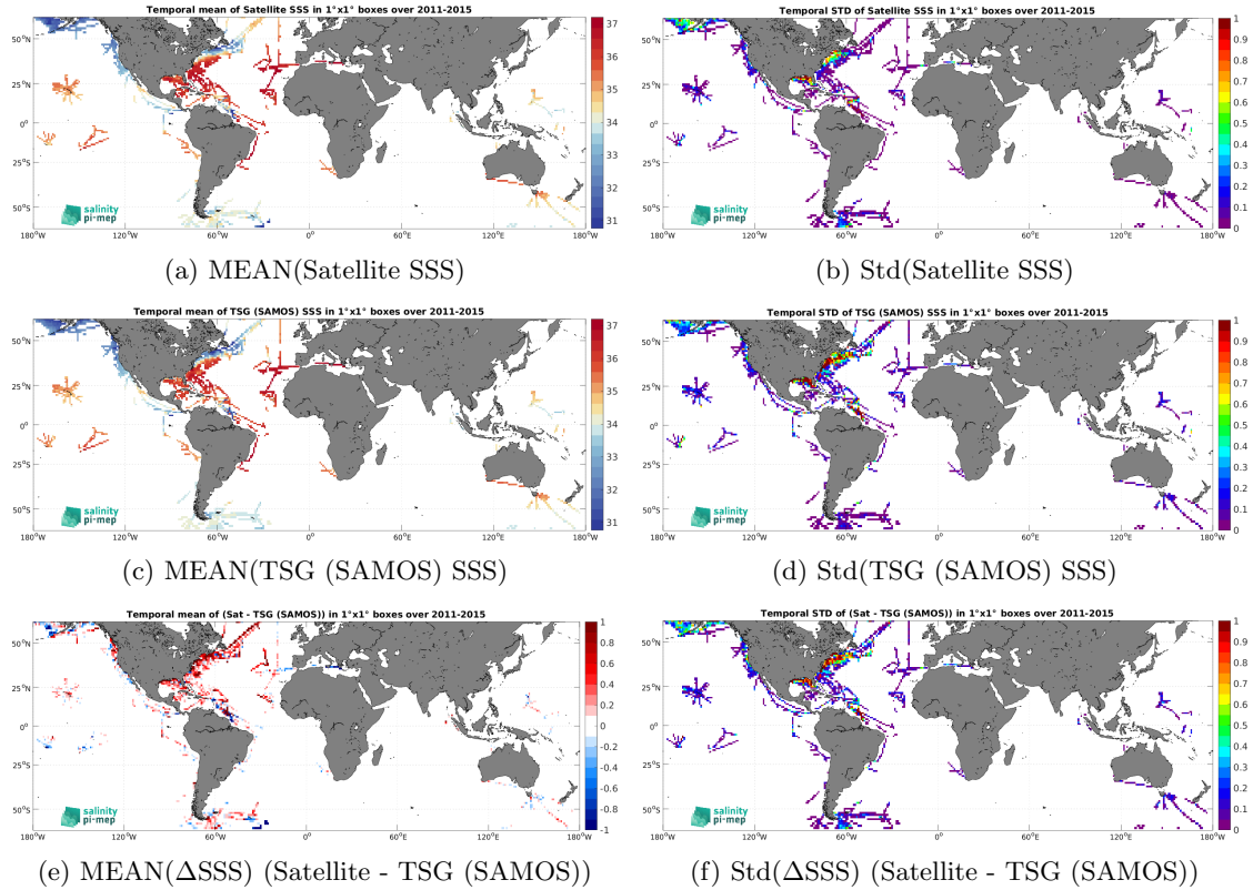
Figure 7: Temporal mean (left) and Std (right) of SSS from Aquarius SSS L3 OR v5 - Monthly - Rain mask (NASA-GSFC) (top), TSG (SAMOS) (middle), and of \Delta SSS (Satellite - TSG (SAMOS)). Only match-up pairs are used to generate these maps.
