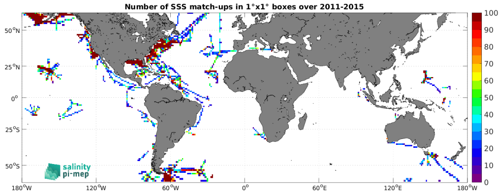
Figure 5: Number of SSS match-ups between TSG (SAMOS) SSS and the Aquarius SSS L3 OR v5 - Monthly - Rain mask (NASA-GSFC) SSS product for the SMOS coastal zone (<800km) 60N-60S Pi-MEP region over 1^{\circ} \times 1^{\circ} boxes and for the full satellite product period.
