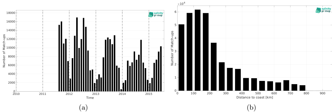
Figure 2: Number of match-ups between TSG (SAMOS) and Aquarius SSS L3 OR v5 - Monthly - Rain mask (NASA-GSFC) SSS as a function of time (a) and as function of the distance to coast (b) over the SMOS coastal zone ( < 800\text{km} ) 60N-60S Pi-MEP region and for the full satellite product period.
