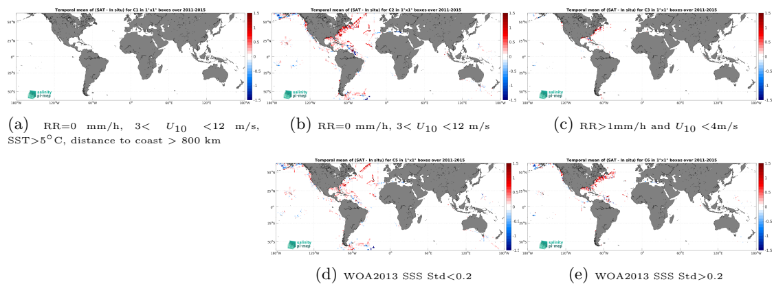
Figure 14: Temporal mean gridded over spatial boxes of size 1^\circ \times 1^\circ of \Delta\text{SSS} (Aquarius SSS L3 OR v5 - Monthly - Rain mask (NASA-GSFC) - TSG (SAMOS)) for 5 different subdatasets corresponding to:RR=0 mm/h, 3 < U_{10} < 12 m/s, SST>5°C, distance to coast > 800 km (a), RR=0 mm/h, 3 < U_{10} < 12 m/s (b), RR>1mm/h and U_{10} < 4 m/s (c), WOA2013 SSS Std<0.2 (d), WOA2013 SSS Std>0.2 (e).
