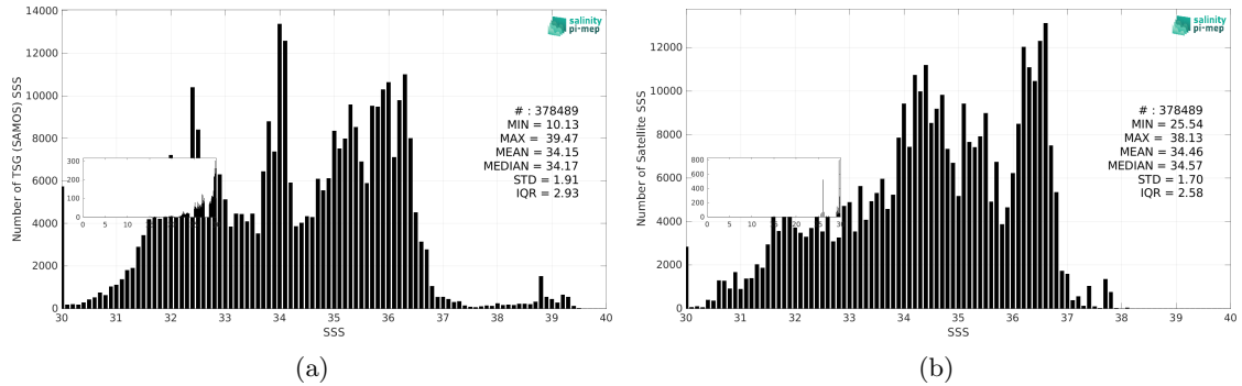
Figure 3: Histograms of SSS from TSG (SAMOS) (a) and Aquarius SSS L3 OR v5 - Monthly - Rain mask (NASA-GSFC) (b) considering all match-up pairs per bins of 0.1 over the SMOS coastal zone (<800km) 60N-60S Pi-MEP region and for the full satellite product period.
