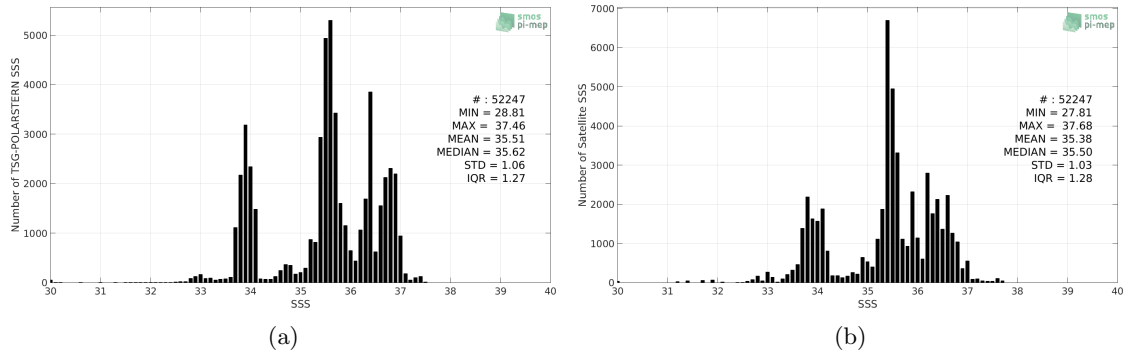
Figure 2: Histograms of SSS from TSG-POLARSTERN (a) and Aquarius-L3-OR-V5-MONTHLY-RAIN-MASK-1DEG (b) considering all match-up pairs per bins of 0.1 over the SMOS coastal zone ( \pm 800\text{km} ) 60N-60S Pi-MEP region and for the full satellite product period.
