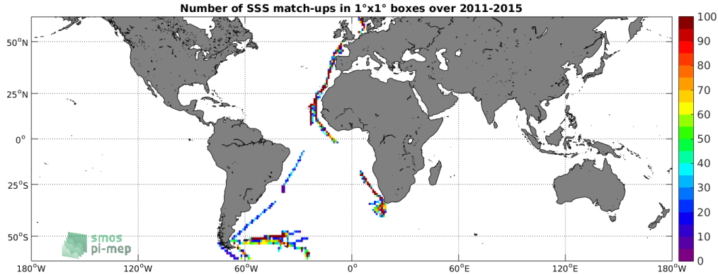
Figure 4: Number of SSS match-ups between TSG-POLARSTERN SSS and the Aquarius-L3-OR-V5-MONTHLY-RAIN-MASK-1DEG SSS product for the SMOS coastal zone ( \approx 800\text{km} ) 60N-60S Pi-MEP region over 1^\circ \times 1^\circ boxes and for the full satellite product period.
