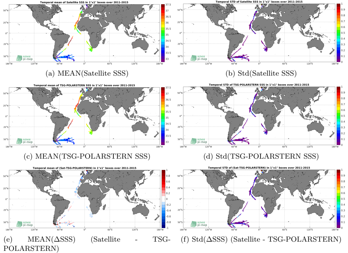
Figure 6: Temporal mean (left) and Std (right) of SSS from Aquarius-L3-OR-V5-MONTHLY-RAIN-MASK-1DEG (top), TSG-POLARSTERN (middle), and of \Delta SSS (Satellite - TSG-POLARSTERN). Only match-up pairs are used to generate these maps.
