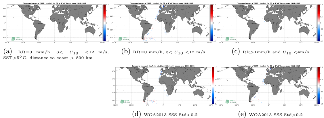
Figure 12: Temporal mean gridded over spatial boxes of size 1^\circ \times 1^\circ of \Delta SSS (Aquarius-L3-OR-V5-MONTHLY-RAIN-MASK-1DEG - TSG-POLARSTERN) for 5 different subdatasets corresponding to:RR=0 mm/h, 3 < U_{10} < 12 m/s, SST >5^\circ\text{C} , distance to coast > 800 km (a), RR=0 mm/h, 3 < U_{10} < 12 m/s (b), RR >1 mm/h and U_{10} < 4 m/s (c), WOA2013 SSS Std <0.2 (d), WOA2013 SSS Std >0.2 (e).
