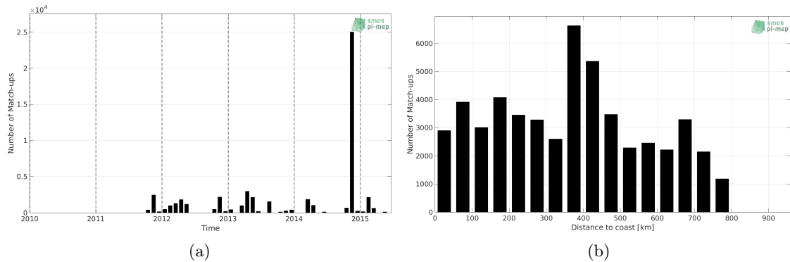
Figure 1: Number of match-ups between TSG-POLARSTERN and Aquarius-L3-OR-V5-MONTHLY-RAIN-MASK-1DEG SSS as a function of time (a) and as function of the distance to coast (b) over the SMOS coastal zone ( \pm 800 km) 60N-60S Pi-MEP region and for the full satellite product period.
