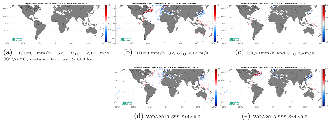
Figure 14: Temporal mean gridded over spatial boxes of size 1^\circ \times 1^\circ of \Delta SSS (Aquarius SSS L3 OR v5 - Monthly - Rain mask (NASA-GSFC) - TSG (LEGOS-DM)) for 5 different subdatasets corresponding to: RR=0 mm/h, 3 < U_{10} < 12 m/s, SST > 5°C, distance to coast > 800 km (a), RR=0 mm/h, 3 < U_{10} < 12 m/s (b), RR > 1mm/h and U_{10} < 4 m/s (c), WOA2013 SSS Std < 0.2 (d), WOA2013 SSS Std > 0.2 (e).
