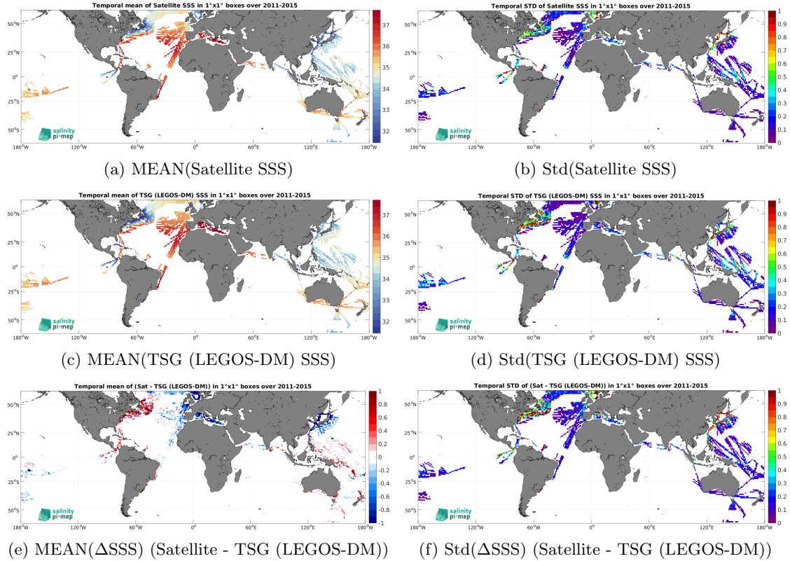
Figure 7: Temporal mean (left) and Std (right) of SSS from Aquarius SSS L3 OR v5 - Monthly - Rain mask (NASA-GSFC) (top), TSG (LEGOS-DM) (middle), and of \Delta\text{SSS} (Satellite - TSG (LEGOS-DM)). Only match-up pairs are used to generate these maps.
