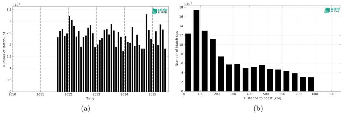
Figure 2: Number of match-ups between TSG (LEGOS-DM) and Aquarius SSS L3 OR v5 - Monthly - Rain mask (NASA-GSFC) SSS as a function of time (a) and as function of the distance to coast (b) over the SMOS coastal zone (<800km) 60N-60S Pi-MEP region and for the full satellite product period.
