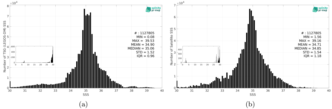
Figure 3: Histograms of SSS from TSG (LEGOS-DM) (a) and Aquarius SSS L3 OR v5 - Monthly - Rain mask (NASA-GSFC) (b) considering all match-up pairs per bins of 0.1 over the SMOS coastal zone (<800km) 60N-60S Pi-MEP region and for the full satellite product period.
