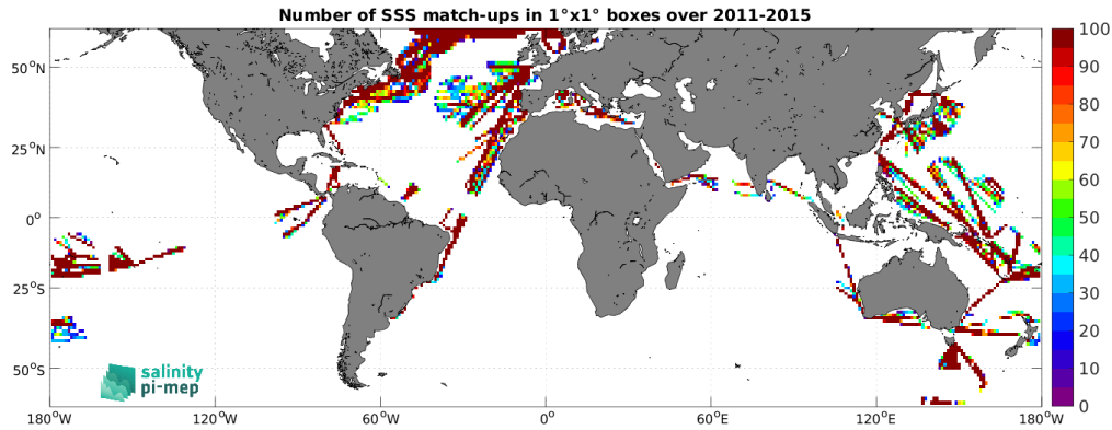
Figure 4: Number of SSS match-ups between TSG (LEGOS-DM) SSS and the Aquarius SSS L3 OR v5 - Monthly - Rain mask (NASA-GSFC) SSS product for the SMOS coastal zone ( <800\text{km} ) 60N-60S Pi-MEP region over 1^\circ \times 1^\circ boxes and for the full satellite product period.
