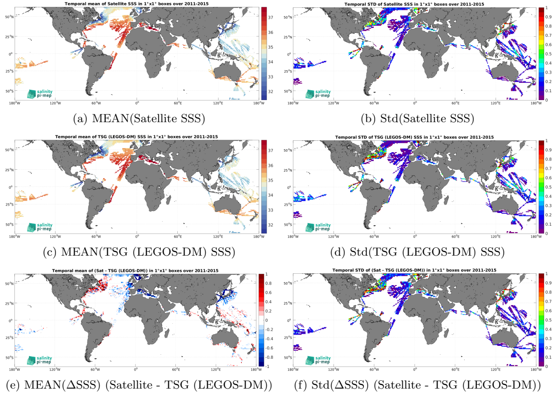
Figure 6: Temporal mean (left) and Std (right) of SSS from Aquarius SSS L3 OR v5 - Monthly - Rain mask (NASA-GSFC) (top), TSG (LEGOS-DM) (middle), and of \Delta\text{SSS} (Satellite - TSG (LEGOS-DM)). Only match-up pairs are used to generate these maps.
