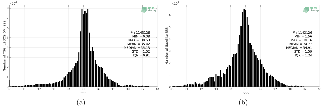
Figure 2: Histograms of SSS from TSG (LEGOS-DM) (a) and Aquarius SSS L3 OR v5 - Monthly - Rain mask (NASA-GSFC) (b) considering all match-up pairs per bins of 0.1 over the SMOS coastal zone (<800km) 60N-60S Pi-MEP region and for the full satellite product period.
