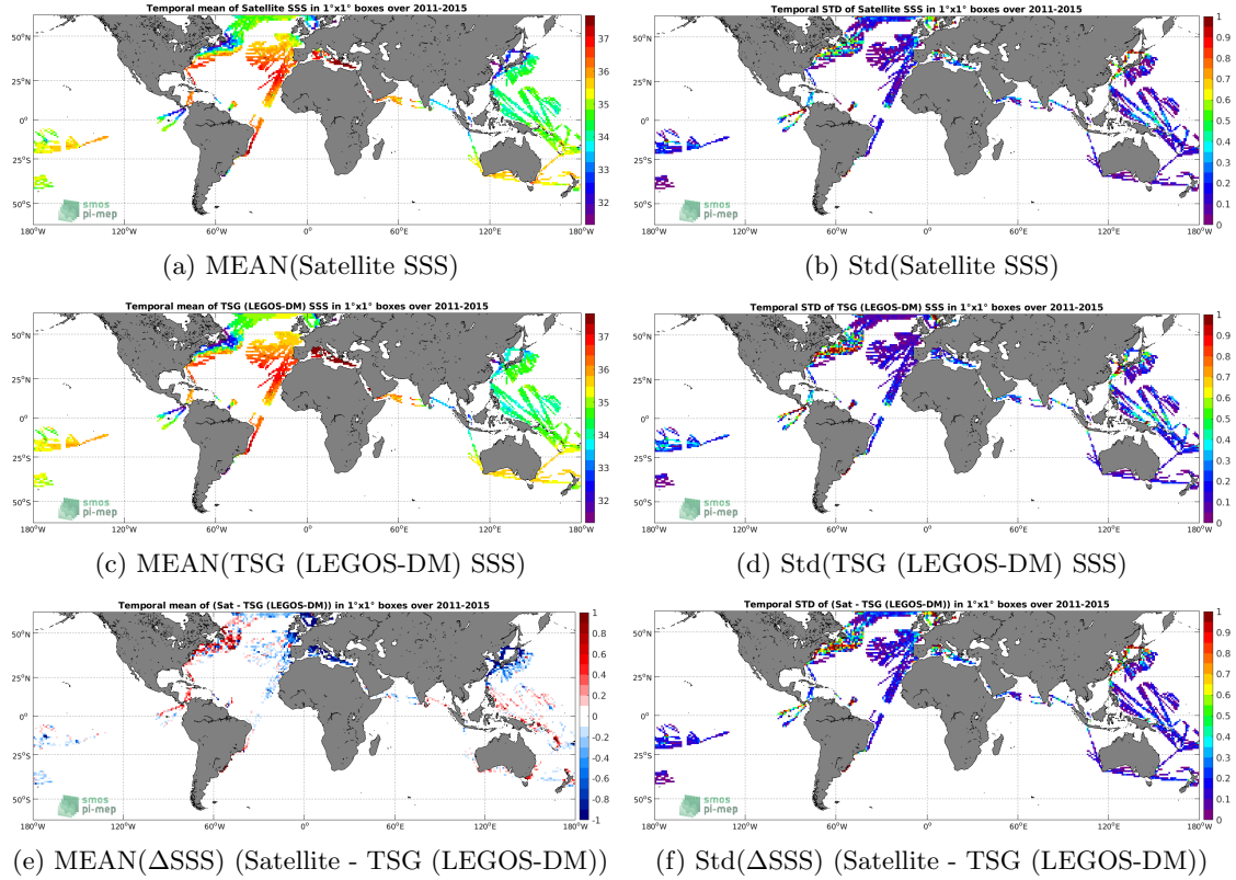
Figure 6: Temporal mean (left) and Std (right) of SSS from Aquarius SSS L3 OR v5 - Monthly - Rain mask (NASA-GSFC) (top), TSG (LEGOS-DM) (middle), and of \Delta SSS (Satellite - TSG (LEGOS-DM)). Only match-up pairs are used to generate these maps.
