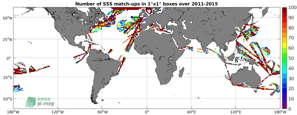
Figure 4: Number of SSS match-ups between TSG (LEGOS-DM) SSS and the Aquarius SSS L3 OR v5 - Monthly - Rain mask (NASA-GSFC) SSS product for the SMOS coastal zone (<800km) 60N-60S Pi-MEP region over 1^\circ \times 1^\circ boxes and for the full satellite product period.
