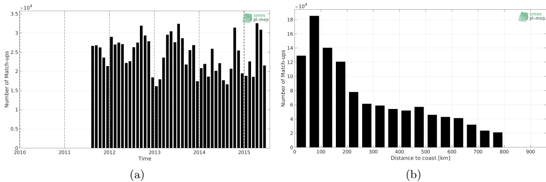
Figure 1: Number of match-ups between TSG (LEGOS-DM) and Aquarius SSS L3 OR v5 - Monthly - Rain mask (NASA-GSFC) SSS as a function of time (a) and as function of the distance to coast (b) over the SMOS coastal zone (<800km) 60N-60S Pi-MEP region and for the full satellite product period.
