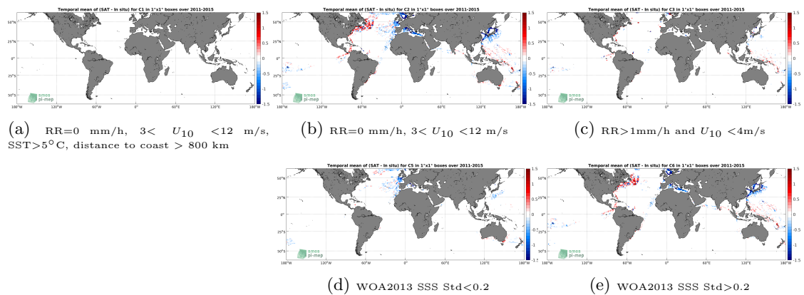
Figure 12: Temporal mean gridded over spatial boxes of size 1^\circ \times 1^\circ of \Delta SSS (Aquarius SSS L3 OR v5 - Monthly - Rain mask (NASA-GSFC) - TSG (LEGOS-DM)) for 5 different subdatasets corresponding to:RR=0 mm/h, 3 < U_{10} < 12 m/s, SST >5^\circ\text{C} , distance to coast > 800 km (a), RR=0 mm/h, 3 < U_{10} < 12 m/s (b), RR >1 mm/h and U_{10} < 4 m/s (c), WOA2013 SSS Std <0.2 (d), WOA2013 SSS Std >0.2 (e).
