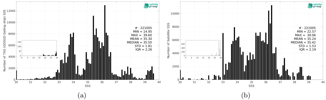
Figure 3: Histograms of SSS from TSG (GOSUD-Sailing-ship) (a) and Aquarius SSS L3 OR v5 - Monthly - Rain mask (NASA-GSFC) (b) considering all match-up pairs per bins of 0.1 over the SMOS coastal zone (<800km) 60N-60S Pi-MEP region and for the full satellite product period.
