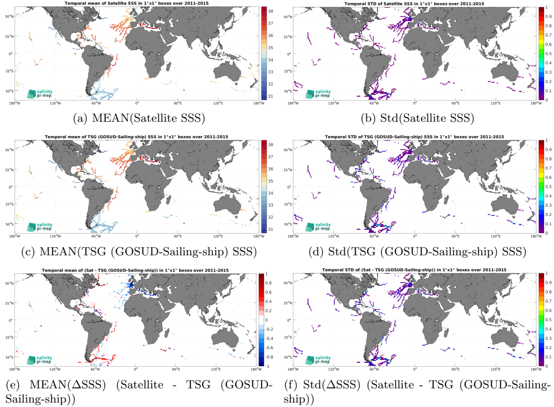
Figure 7: Temporal mean (left) and Std (right) of SSS from Aquarius SSS L3 OR v5 - Monthly - Rain mask (NASA-GSFC) (top), TSG (GOSUD-Sailing-ship) (middle), and of \Delta\text{SSS} (Satellite - TSG (GOSUD-Sailing-ship)). Only match-up pairs are used to generate these maps.
