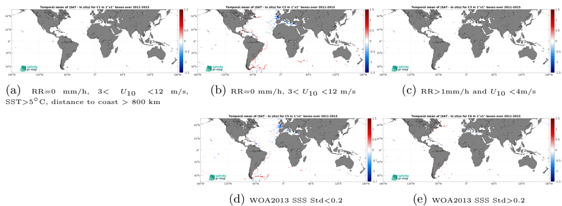
Figure 14: Temporal mean gridded over spatial boxes of size 1^\circ \times 1^\circ of \Delta\text{SSS} (Aquarius SSS L3 OR v5 - Monthly - Rain mask (NASA-GSFC) - TSG (GOSUD-Sailing-ship)) for 5 different subdatasets corresponding to:RR=0 mm/h, 3 < U_{10} < 12 m/s, SST > 5^\circ\text{C} , distance to coast > 800 km (a), RR=0 mm/h, 3 < U_{10} < 12 m/s (b), RR > 1 mm/h and U_{10} < 4 m/s (c), WOA2013 SSS Std < 0.2 (d), WOA2013 SSS Std > 0.2 (e).
