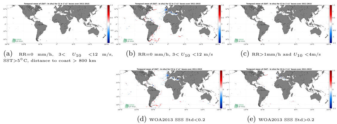
Figure 12: Temporal mean gridded over spatial boxes of size 1^\circ \times 1^\circ of \Delta SSS (Aquarius SSS L3 OR v5 - Monthly - Rain mask (NASA-GSFC) - TSG (GOSUD-Sailing-ship)) for 5 different subdatasets corresponding to:RR=0 mm/h, 3 < U_{10} < 12 m/s, SST >5^\circ C, distance to coast > 800 km (a), RR=0 mm/h, 3 < U_{10} < 12 m/s (b), RR >1 mm/h and U_{10} < 4 m/s (c), WOA2013 SSS Std <0.2 (d), WOA2013 SSS Std >0.2 (e).
