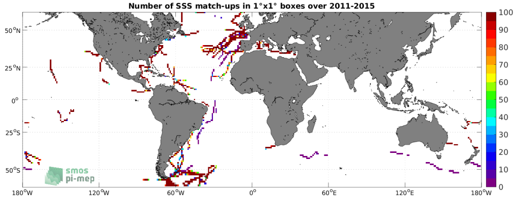
Figure 4: Number of SSS match-ups between TSG (GOSUD-Sailing-ship) SSS and the Aquarius SSS L3 OR v5 - Monthly - Rain mask (NASA-GSFC) SSS product for the SMOS coastal zone (<800km) 60N-60S Pi-MEP region over 1^\circ \times 1^\circ boxes and for the full satellite product period.
