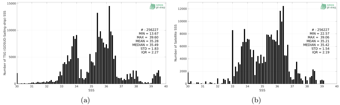
Figure 2: Histograms of SSS from TSG (GOSUD-Sailing-ship) (a) and Aquarius SSS L3 OR v5 - Monthly - Rain mask (NASA-GSFC) (b) considering all match-up pairs per bins of 0.1 over the SMOS coastal zone (<800km) 60N-60S Pi-MEP region and for the full satellite product period.
