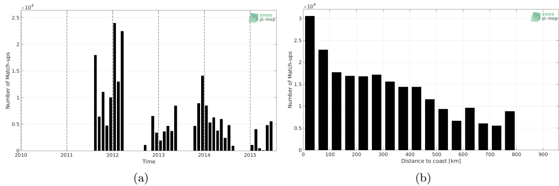
Figure 1: Number of match-ups between TSG-GOSUD-Sailing-ship and Aquarius-L3-OR-V5-MONTHLY-RAIN-MASK-1DEG SSS as a function of time (a) and as function of the distance to coast (b) over the SMOS coastal zone ( \approx 800 km) 60N-60S Pi-MEP region and for the full satellite product period.
