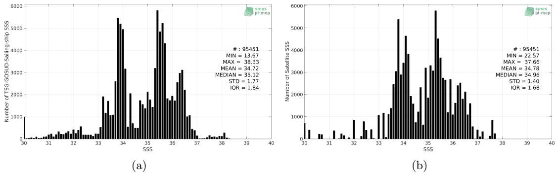
Figure 2: Histograms of SSS from TSG-GOSUD-Sailing-ship (a) and Aquarius-L3-OR-V5-MONTHLY-RAIN-MASK-1DEG (b) considering all match-up pairs per bins of 0.1 over the SMOS coastal zone ( \approx 800 km) 60N-60S Pi-MEP region and for the full satellite product period.
