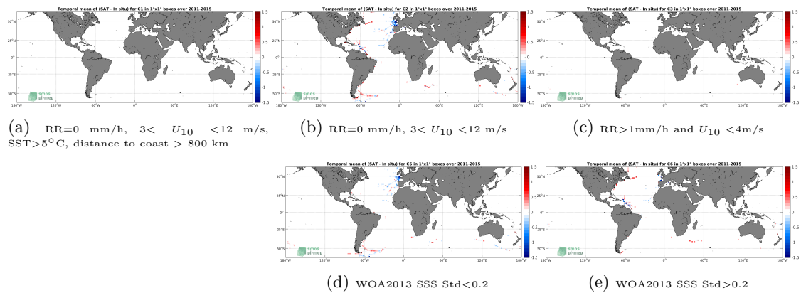
Figure 12: Temporal mean gridded over spatial boxes of size 1^\circ \times 1^\circ of \Delta SSS (Aquarius-L3-OR-V5-MONTHLY-RAIN-MASK-1DEG - TSG-GOSUD-Sailing-ship) for 5 different subdatasets corresponding to:RR=0 mm/h, 3 < U_{10} < 12 m/s, SST >5^\circ C, distance to coast > 800 km (a), RR=0 mm/h, 3 < U_{10} < 12 m/s (b), RR >1 mm/h and U_{10} < 4 m/s (c), WOA2013 SSS Std <0.2 (d), WOA2013 SSS Std >0.2 (e).
