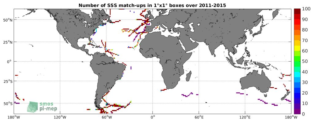
Figure 4: Number of SSS match-ups between TSG-GOSUD-Sailing-ship SSS and the Aquarius-L3-OR-V5-MONTHLY-RAIN-MASK-1DEG SSS product for the SMOS coastal zone ( \pm 800\text{km} ) 60N-60S Pi-MEP region over 1^\circ \times 1^\circ boxes and for the full satellite product period.
