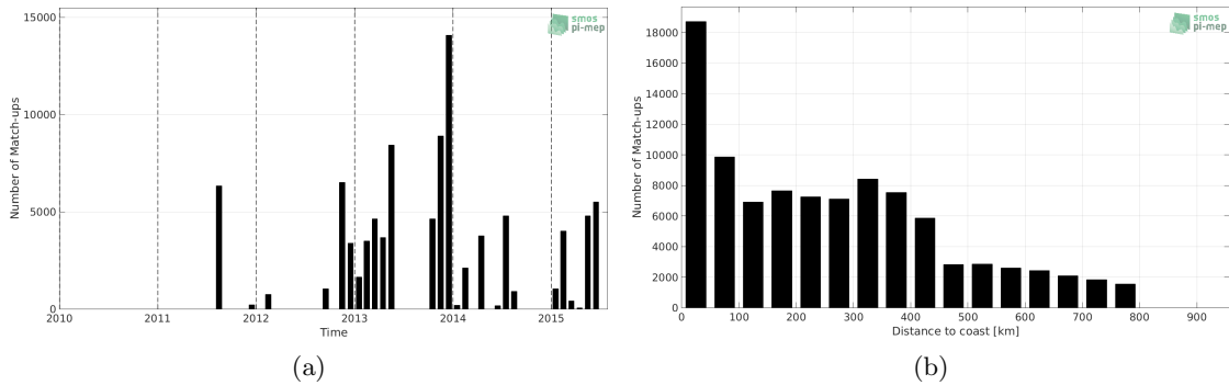
Figure 1: Number of match-ups between TSG-GOSUD-Sailing-ship and Aquarius-L3-OR-V5-MONTHLY-RAIN-MASK-1DEG SSS as a function of time (a) and as function of the distance to coast (b) over the SMOS coastal zone ( \approx 800 km) 60N-60S Pi-MEP region and for the full satellite product period.
