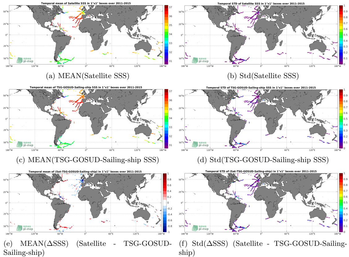
Figure 6: Temporal mean (left) and Std (right) of SSS from Aquarius-L3-OR-V5-MONTHLY-RAIN-MASK-1DEG (top), TSG-GOSUD-Sailing-ship (middle), and of \Delta SSS (Satellite - TSG-GOSUD-Sailing-ship). Only match-up pairs are used to generate these maps.
