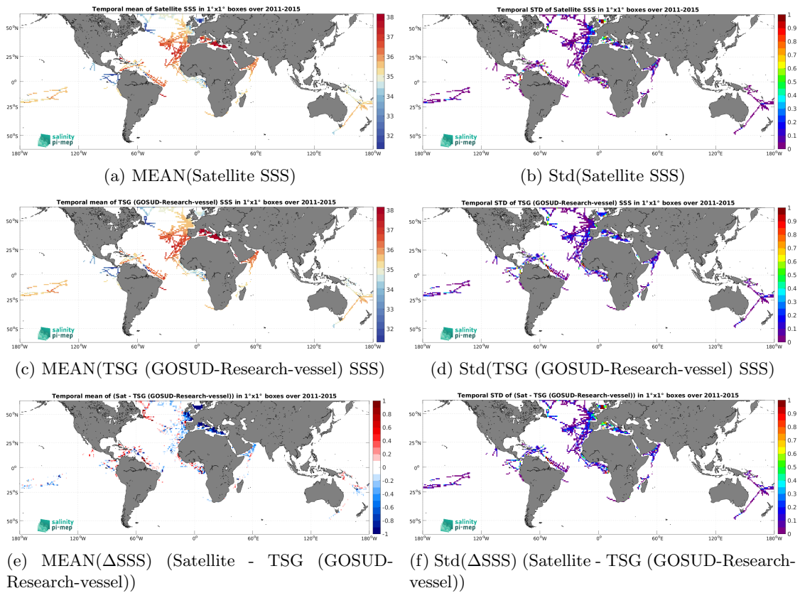
Figure 7: Temporal mean (left) and Std (right) of SSS from Aquarius SSS L3 OR v5 - Monthly - Rain mask (NASA-GSFC) (top), TSG (GOSUD-Research-vessel) (middle), and of \Delta SSS (Satellite - TSG (GOSUD-Research-vessel)). Only match-up pairs are used to generate these maps.
