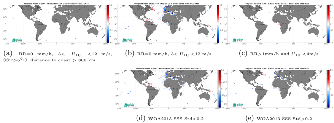
Figure 14: Temporal mean gridded over spatial boxes of size 1^\circ \times 1^\circ of \Delta SSS (Aquarius SSS L3 OR v5 - Monthly - Rain mask (NASA-GSFC) - TSG (GOSUD-Research-vessel)) for 5 different subdatasets corresponding to:RR=0 mm/h, 3 < U_{10} < 12 m/s, SST > 5^\circ\text{C} , distance to coast > 800 km (a), RR=0 mm/h, 3 < U_{10} < 12 m/s (b), RR > 1 mm/h and U_{10} < 4 m/s (c), WOA2013 SSS Std < 0.2 (d), WOA2013 SSS Std > 0.2 (e).
