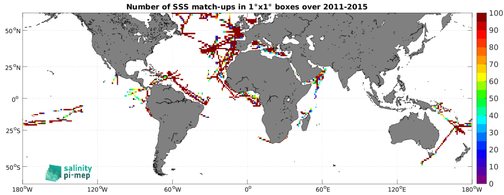
Figure 5: Number of SSS match-ups between TSG (GOSUD-Research-vessel) SSS and the Aquarius SSS L3 OR v5 - Monthly - Rain mask (NASA-GSFC) SSS product for the SMOS coastal zone (<800km) 60N-60S Pi-MEP region over 1^\circ \times 1^\circ boxes and for the full satellite product period.
