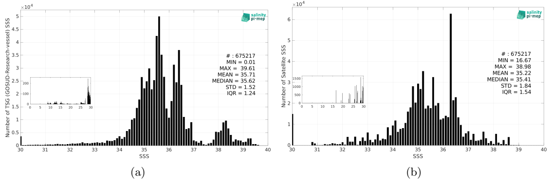
Figure 3: Histograms of SSS from TSG (GOSUD-Research-vessel) (a) and Aquarius SSS L3 OR v5 - Monthly - Rain mask (NASA-GSFC) (b) considering all match-up pairs per bins of 0.1 over the SMOS coastal zone (<800km) 60N-60S Pi-MEP region and for the full satellite product period.
