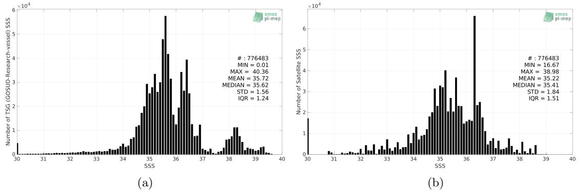
Figure 2: Histograms of SSS from TSG (GOSUD-Research-vessel) (a) and Aquarius SSS L3 OR v5 - Monthly - Rain mask (NASA-GSFC) (b) considering all match-up pairs per bins of 0.1 over the SMOS coastal zone (<800km) 60N-60S Pi-MEP region and for the full satellite product period.
