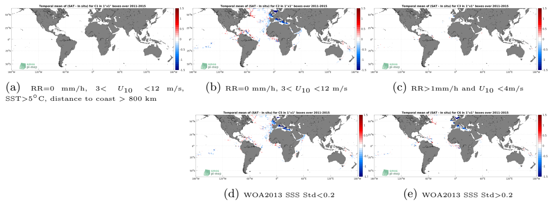
Figure 12: Temporal mean gridded over spatial boxes of size 1^\circ \times 1^\circ of \Delta SSS (Aquarius SSS L3 OR v5 - Monthly - Rain mask (NASA-GSFC) - TSG (GOSUD-Research-vessel)) for 5 different subdatasets corresponding to:RR=0 mm/h, 3 < U_{10} < 12 m/s, SST >5^\circ\text{C} , distance to coast > 800 km (a), RR=0 mm/h, 3 < U_{10} < 12 m/s (b), RR >1 mm/h and U_{10} < 4 m/s (c), WOA2013 SSS Std <0.2 (d), WOA2013 SSS Std >0.2 (e).
