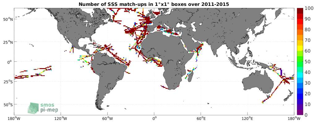
Figure 4: Number of SSS match-ups between TSG (GOSUD-Research-vessel) SSS and the Aquarius SSS L3 OR v5 - Monthly - Rain mask (NASA-GSFC) SSS product for the SMOS coastal zone (<800km) 60N-60S Pi-MEP region over 1^\circ \times 1^\circ boxes and for the full satellite product period.
