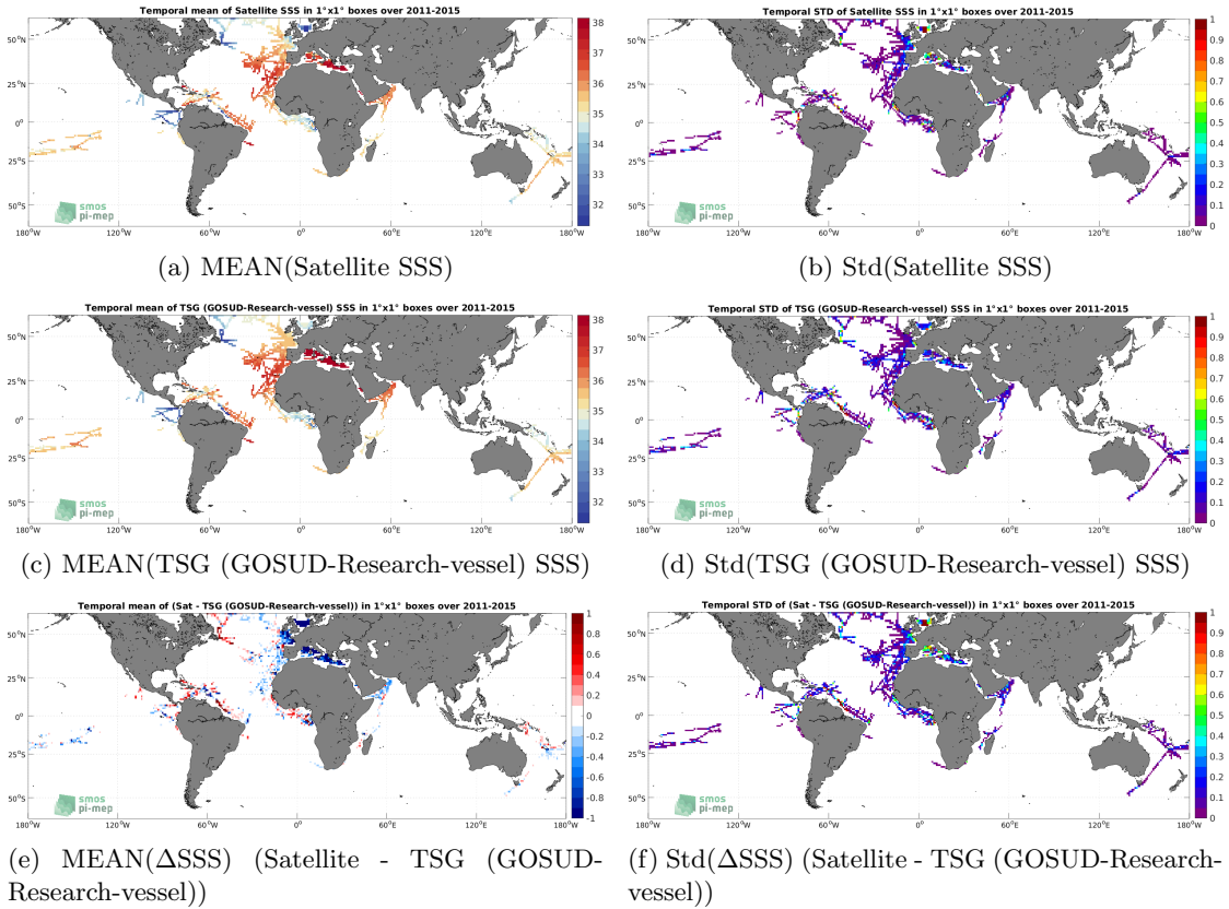
Figure 6: Temporal mean (left) and Std (right) of SSS from Aquarius SSS L3 OR v5 - Monthly - Rain mask (NASA-GSFC) (top), TSG (GOSUD-Research-vessel) (middle), and of \Delta SSS (Satellite - TSG (GOSUD-Research-vessel)). Only match-up pairs are used to generate these maps.
