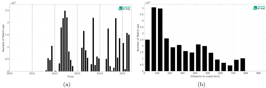
Figure 2: Number of match-ups between TSG (CSIC-UTM) and Aquarius SSS L3 OR v5 - Monthly - Rain mask (NASA-GSFC) SSS as a function of time (a) and as function of the distance to coast (b) over the SMOS coastal zone ( < 800\text{km} ) 60N-60S Pi-MEP region and for the full satellite product period.
