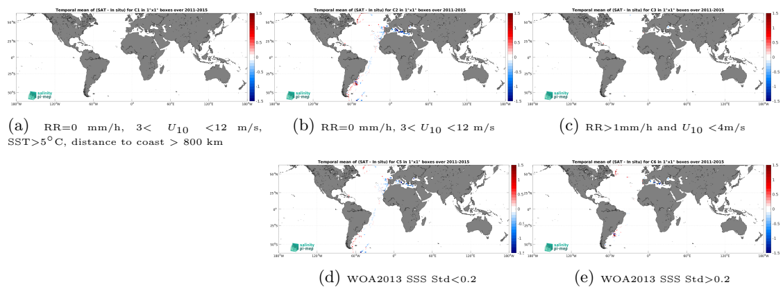
Figure 14: Temporal mean gridded over spatial boxes of size 1^\circ \times 1^\circ of \Delta SSS (Aquarius SSS L3 OR v5 - Monthly - Rain mask (NASA-GSFC) - TSG (CSIC-UTM)) for 5 different subdatasets corresponding to: RR=0 mm/h, 3 < U_{10} < 12 m/s, SST > 5^\circ\text{C} , distance to coast > 800 km (a), RR=0 mm/h, 3 < U_{10} < 12 m/s (b), RR > 1 mm/h and U_{10} < 4 m/s (c), WOA2013 SSS Std < 0.2 (d), WOA2013 SSS Std > 0.2 (e).
