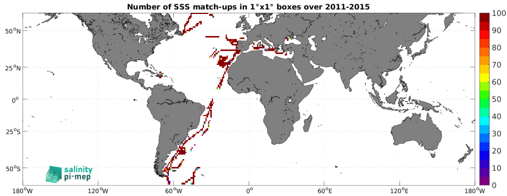
Figure 5: Number of SSS match-ups between TSG (CSIC-UTM) SSS and the Aquarius SSS L3 OR v5 - Monthly - Rain mask (NASA-GSFC) SSS product for the SMOS coastal zone ( <800\text{km} ) 60N-60S Pi-MEP region over 1^\circ \times 1^\circ boxes and for the full satellite product period.
