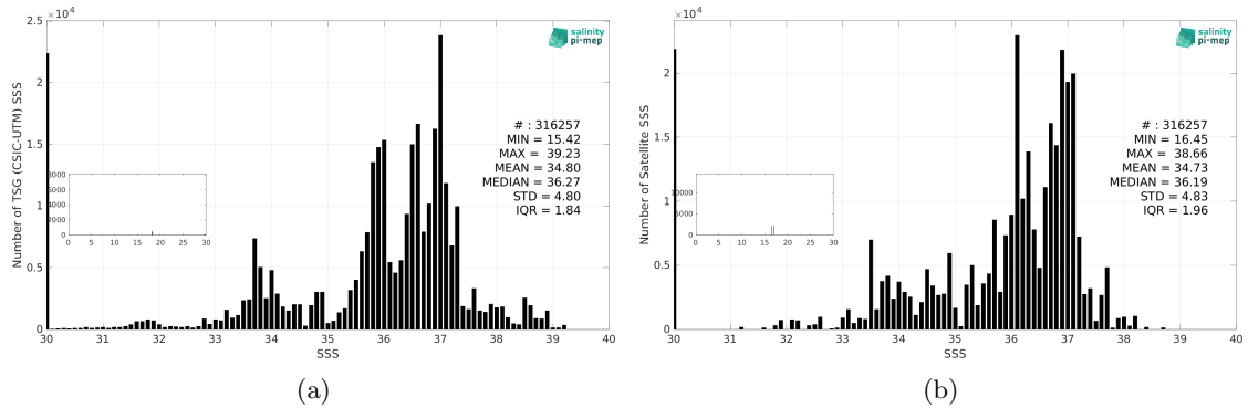
Figure 3: Histograms of SSS from TSG (CSIC-UTM) (a) and Aquarius SSS L3 OR v5 - Monthly - Rain mask (NASA-GSFC) (b) considering all match-up pairs per bins of 0.1 over the SMOS coastal zone (<800km) 60N-60S Pi-MEP region and for the full satellite product period.
