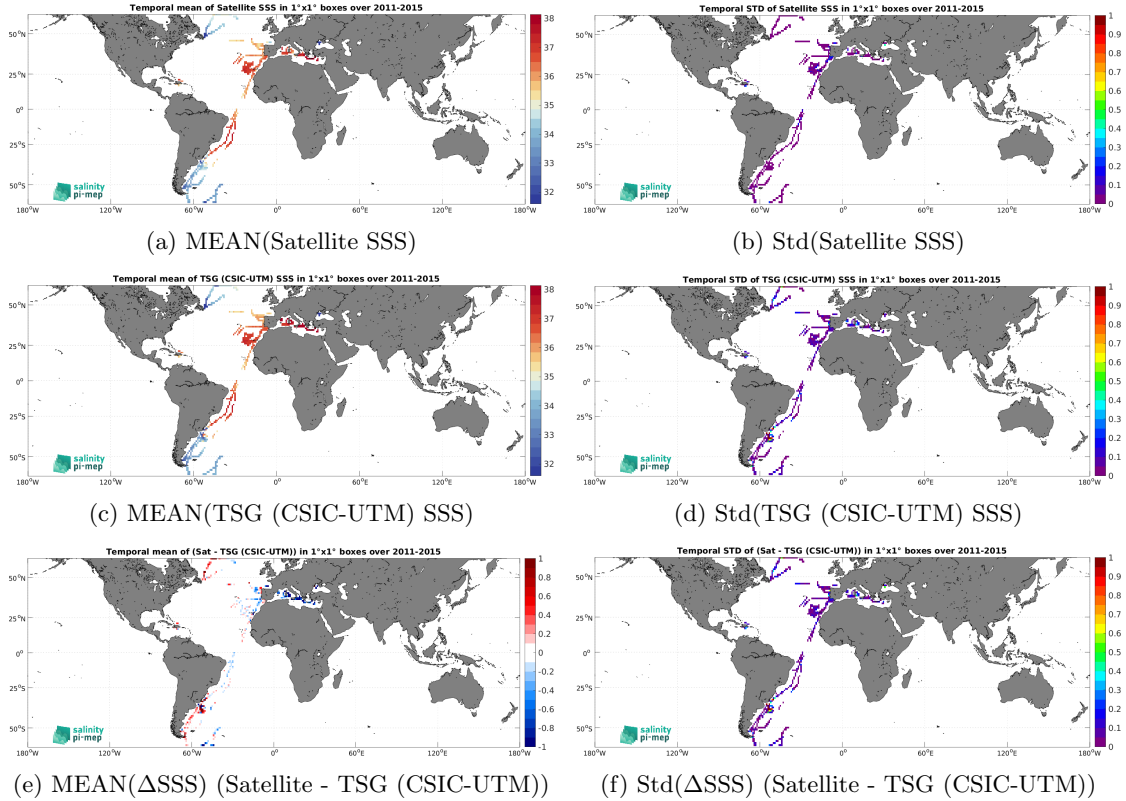
Figure 7: Temporal mean (left) and Std (right) of SSS from Aquarius SSS L3 OR v5 - Monthly - Rain mask (NASA-GSFC) (top), TSG (CSIC-UTM) (middle), and of \Delta\text{SSS} (Satellite - TSG (CSIC-UTM)). Only match-up pairs are used to generate these maps.
