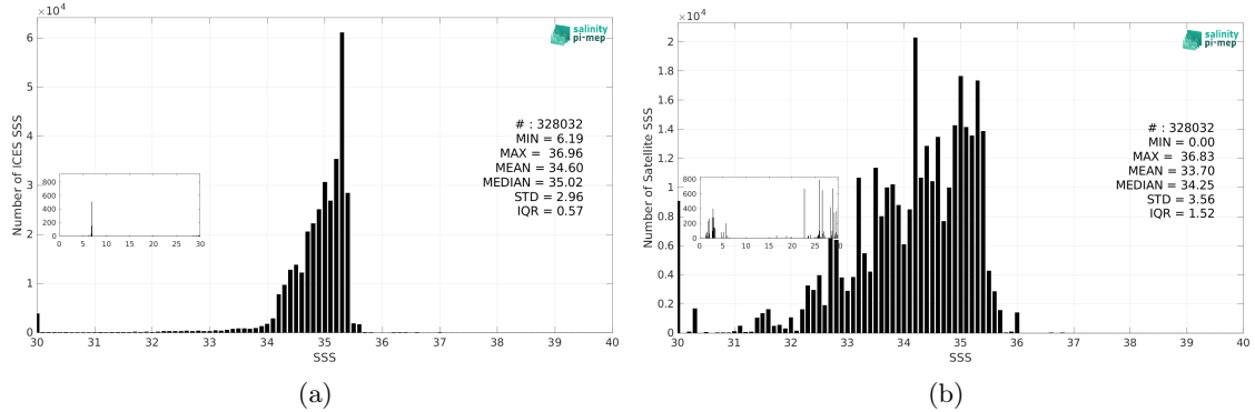
Figure 3: Histograms of SSS from ICES (a) and Aquarius SSS L3 OR v5 - Monthly - Rain mask (NASA-GSFC) (b) considering all match-up pairs per bins of 0.1 over the SMOS coastal zone (<800km) 60N-60S Pi-MEP region and for the full satellite product period.
