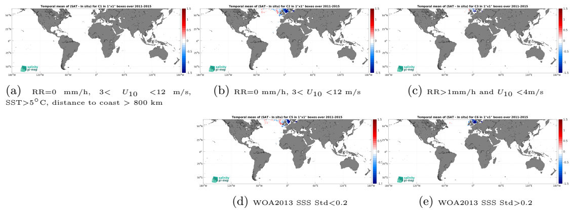
Figure 14: Temporal mean gridded over spatial boxes of size 1^\circ \times 1^\circ of \Delta SSS (Aquarius SSS L3 OR v5 - Monthly - Rain mask (NASA-GSFC) - ICES) for 5 different subdatasets corresponding to:RR=0 mm/h, 3 < U_{10} < 12 m/s, SST >5^\circ C, distance to coast > 800 km (a), RR=0 mm/h, 3 < U_{10} < 12 m/s (b), RR >1 mm/h and U_{10} < 4 m/s (c), WOA2013 SSS Std <0.2 (d), WOA2013 SSS Std >0.2 (e).
