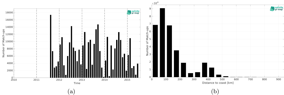
Figure 2: Number of match-ups between ICES and Aquarius SSS L3 OR v5 - Monthly - Rain mask (NASA-GSFC) SSS as a function of time (a) and as function of the distance to coast (b) over the SMOS coastal zone (<800km) 60N-60S Pi-MEP region and for the full satellite product period.
