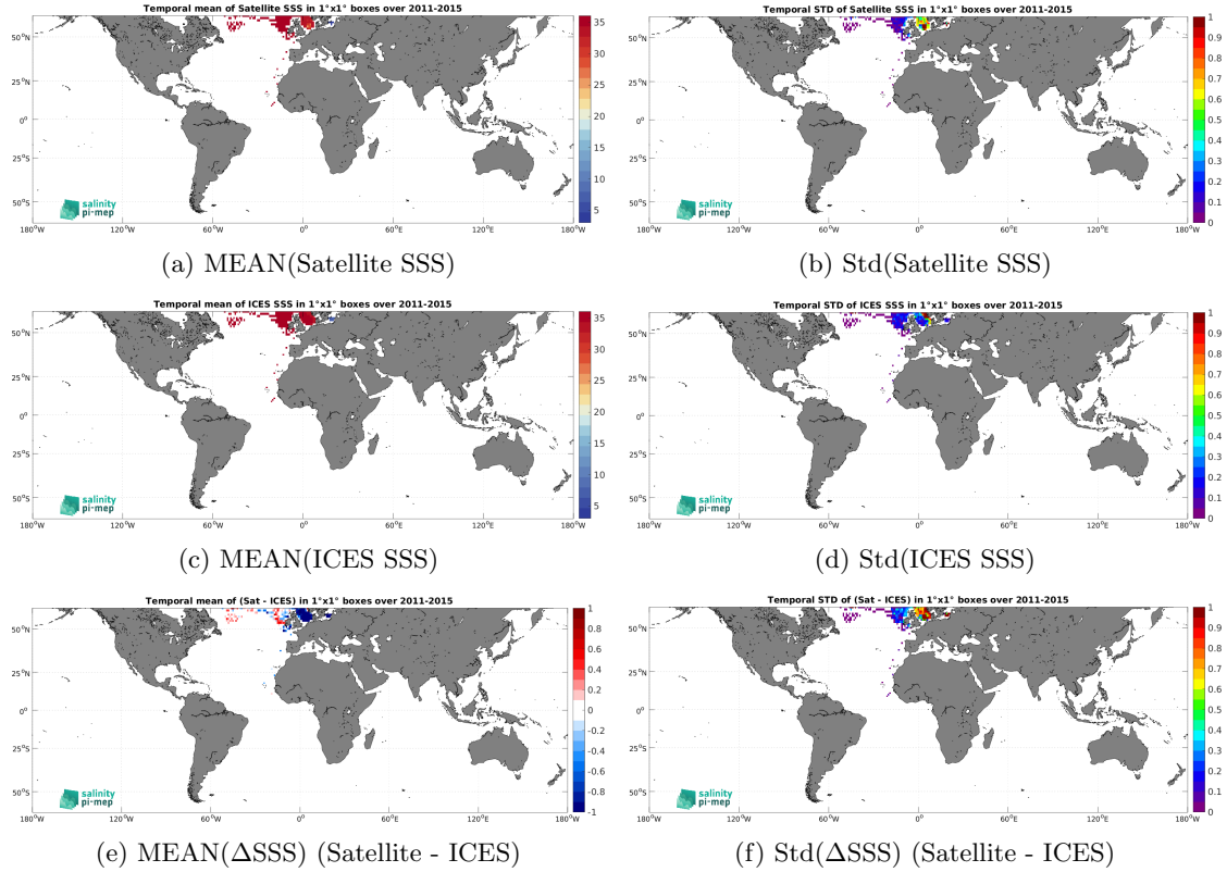
Figure 7: Temporal mean (left) and Std (right) of SSS from Aquarius SSS L3 OR v5 - Monthly - Rain mask (NASA-GSFC) (top), ICES (middle), and of \Delta SSS (Satellite - ICES). Only match-up pairs are used to generate these maps.
