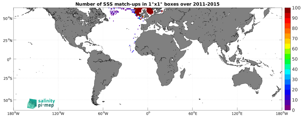
Figure 4: Number of SSS match-ups between ICES SSS and the Aquarius SSS L3 OR v5 - Monthly - Rain mask (NASA-GSFC) SSS product for the SMOS coastal zone (<800km) 60N-60S Pi-MEP region over 1^\circ \times 1^\circ boxes and for the full satellite product period.
