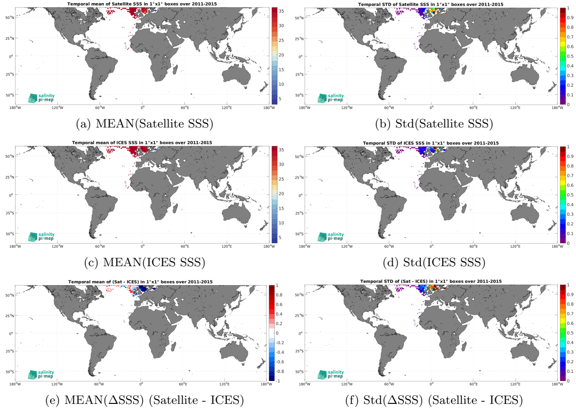
Figure 6: Temporal mean (left) and Std (right) of SSS from Aquarius SSS L3 OR v5 - Monthly - Rain mask (NASA-GSFC) (top), ICES (middle), and of \Delta SSS (Satellite - ICES). Only match-up pairs are used to generate these maps.
