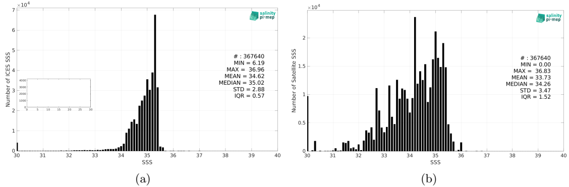
Figure 2: Histograms of SSS from ICES (a) and Aquarius SSS L3 OR v5 - Monthly - Rain mask (NASA-GSFC) (b) considering all match-up pairs per bins of 0.1 over the SMOS coastal zone (<800km) 60N-60S Pi-MEP region and for the full satellite product period.
