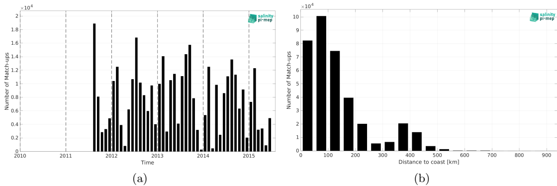
Figure 1: Number of match-ups between ICES and Aquarius SSS L3 OR v5 - Monthly - Rain mask (NASA-GSFC) SSS as a function of time (a) and as function of the distance to coast (b) over the SMOS coastal zone (<800km) 60N-60S Pi-MEP region and for the full satellite product period.
