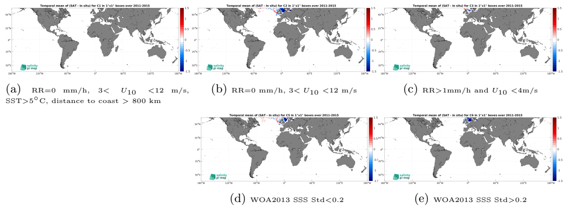
Figure 12: Temporal mean gridded over spatial boxes of size 1^\circ \times 1^\circ of \Delta SSS (Aquarius SSS L3 OR v5 - Monthly - Rain mask (NASA-GSFC) - ICES) for 5 different subdatasets corresponding to:RR=0 mm/h, 3 < U_{10} < 12 m/s, SST >5^\circ\text{C} , distance to coast > 800 km (a), RR=0 mm/h, 3 < U_{10} < 12 m/s (b), RR >1 mm/h and U_{10} < 4 m/s (c), WOA2013 SSS Std <0.2 (d), WOA2013 SSS Std >0.2 (e).
