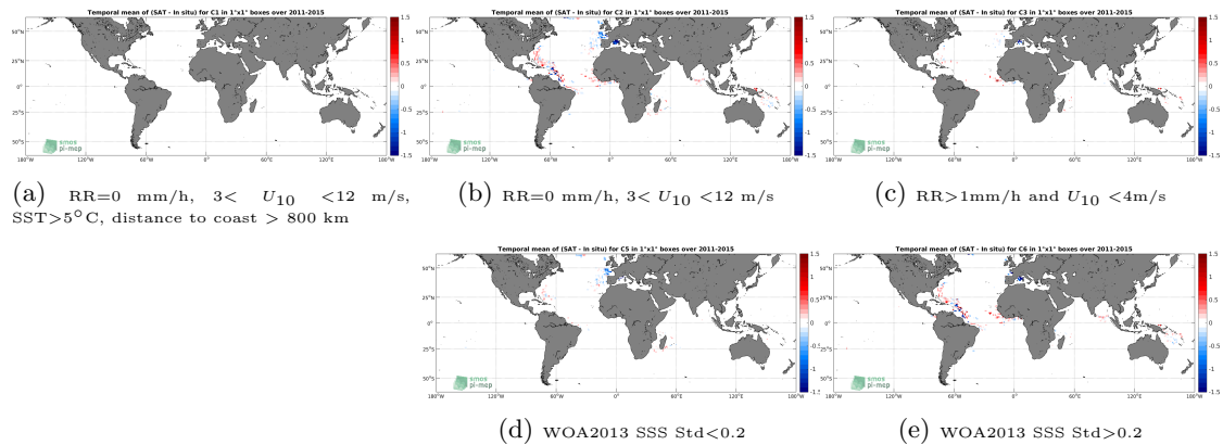
Figure 11: Temporal mean gridded over spatial boxes of size 1^\circ \times 1^\circ of \Delta SSS (Aquarius-L3-OR-V5-MONTHLY-RAIN-MASK-1DEG - Surface drifters) for 5 different subdatasets corresponding to:RR=0 mm/h, 3 < U_{10} < 12 m/s, SST >5^\circ C, distance to coast > 800 km (a), RR=0 mm/h, 3 < U_{10} < 12 m/s (b), RR >1 mm/h and U_{10} < 4 m/s (c), WOA2013 SSS Std <0.2 (d), WOA2013 SSS Std >0.2 (e).
