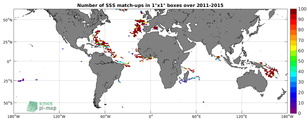
Figure 3: Number of SSS match-ups between Surface drifters SSS and the Aquarius-L3-OR-V5-MONTHLY-RAIN-MASK-1DEG SSS product for the SMOS coastal zone ( \approx 800\text{km} ) 60N-60S Pi-MEP region over 1°x1° boxes and for the full satellite product period.
