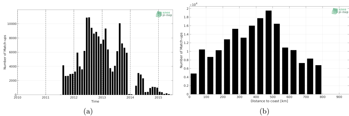
Figure 1: Number of match-ups between Surface drifters and Aquarius-L3-OR-V5-MONTHLY-RAIN-MASK-1DEG SSS as a function of time (a) and as function of the distance to coast (b) over the SMOS coastal zone ( \approx 800 km) 60N-60S Pi-MEP region and for the full satellite product period.
