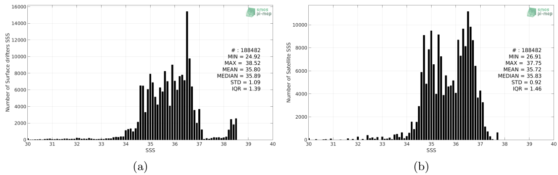
Figure 2: Histograms of SSS from Surface drifters (a) and Aquarius-L3-OR-V5-MONTHLY-RAIN-MASK-1DEG (b) considering all match-up pairs per bins of 0.1 over the SMOS coastal zone ( \approx 800\text{km} ) 60N-60S Pi-MEP region and for the full satellite product period.
