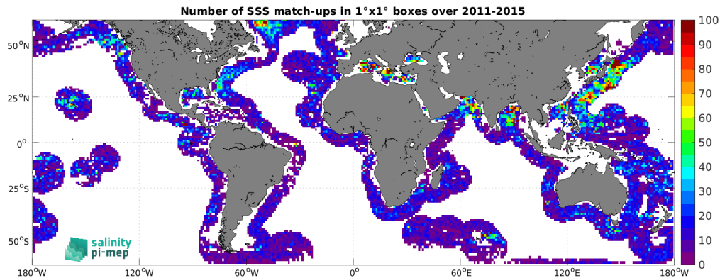
Figure 5: Number of SSS match-ups between Argo SSS and the Aquarius SSS L3 OR v5 - Monthly - Rain mask (NASA-GSFC) SSS product for the SMOS coastal zone (<800km) 60N-60S Pi-MEP region over 1^\circ \times 1^\circ boxes and for the full satellite product period.
