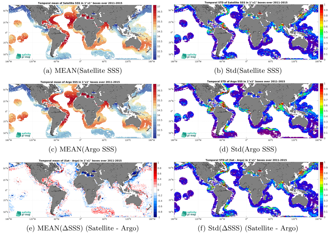
Figure 7: Temporal mean (left) and Std (right) of SSS from Aquarius SSS L3 OR v5 - Monthly - Rain mask (NASA-GSFC) (top), Argo (middle), and of \Delta SSS (Satellite - Argo). Only match-up pairs are used to generate these maps.
