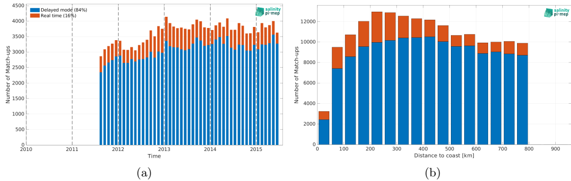
Figure 2: Number of match-ups between Argo and Aquarius SSS L3 OR v5 - Monthly - Rain mask (NASA-GSFC) SSS as a function of time (a) and as function of the distance to coast (b) over the SMOS coastal zone (<800km) 60N-60S Pi-MEP region and for the full satellite product period.
