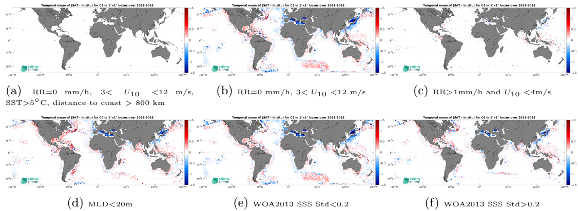
Figure 14: Temporal mean gridded over spatial boxes of size 1^\circ \times 1^\circ of \Delta SSS (Aquarius SSS L3 OR v5 - Monthly - Rain mask (NASA-GSFC) - Argo) for 6 different subdatasets corresponding to:RR=0 mm/h, 3 < U_{10} < 12 m/s, SST >5^\circ C, distance to coast > 800 km (a), RR=0 mm/h, 3 < U_{10} < 12 m/s (b), RR >1 mm/h and U_{10} < 4 m/s (c),MLD <20 m (d),WOA2013 SSS Std <0.2 (e),WOA2013 SSS Std >0.2 (f).
