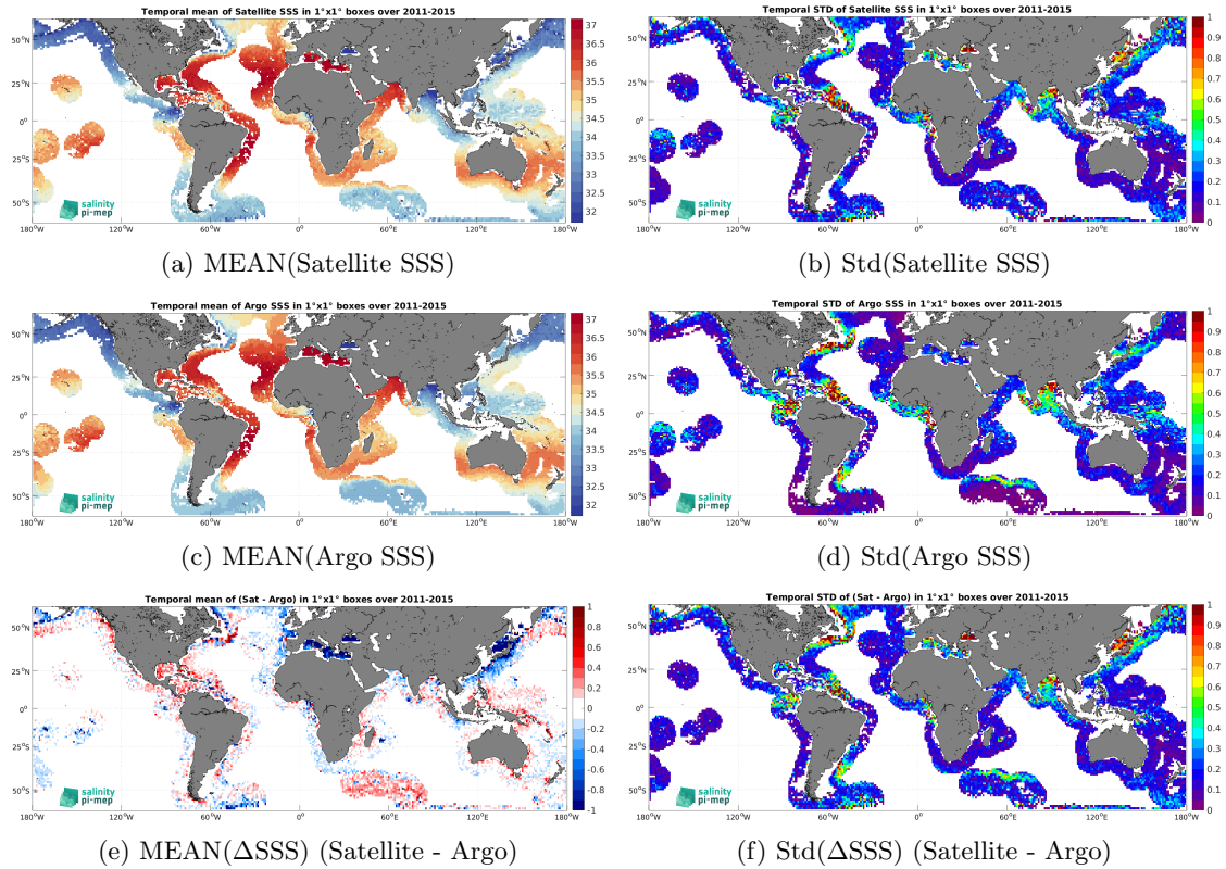
Figure 6: Temporal mean (left) and Std (right) of SSS from Aquarius SSS L3 OR v5 - Monthly - Rain mask (NASA-GSFC) (top), Argo (middle), and of \Delta SSS (Satellite - Argo). Only match-up pairs are used to generate these maps.
