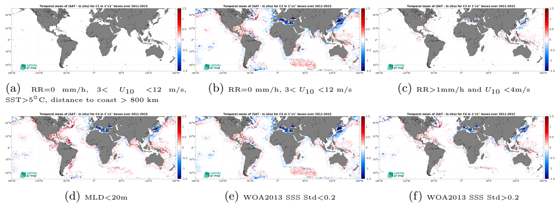
Figure 12: Temporal mean gridded over spatial boxes of size 1^\circ \times 1^\circ of \Delta SSS (Aquarius SSS L3 OR v5 - Monthly - Rain mask (NASA-GSFC) - Argo) for 6 different subdatasets corresponding to:RR=0 mm/h, 3 < U_{10} < 12 m/s, SST > 5^\circ C , distance to coast > 800 km (a), RR=0 mm/h, 3 < U_{10} < 12 m/s (b), RR > 1 mm/h and U_{10} < 4 m/s (c),MLD < 20 m (d),WOA2013 SSS Std < 0.2 (e),WOA2013 SSS Std > 0.2 (f).
