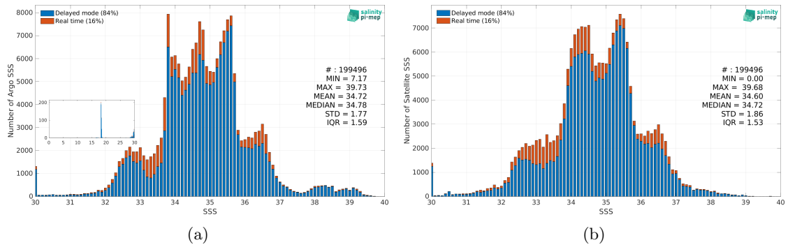
Figure 2: Histograms of SSS from Argo (a) and Aquarius SSS L3 OR v5 - Monthly - Rain mask (NASA-GSFC) (b) considering all match-up pairs per bins of 0.1 over the SMOS coastal zone (<800km) 60N-60S Pi-MEP region and for the full satellite product period.
