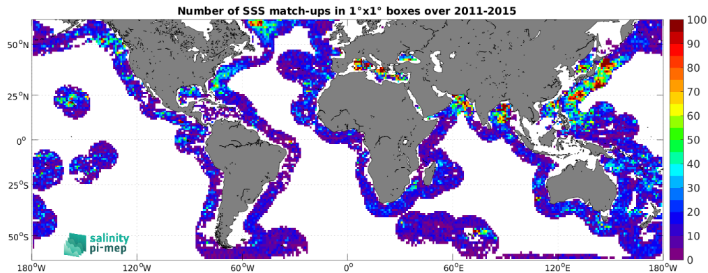
Figure 4: Number of SSS match-ups between Argo SSS and the Aquarius SSS L3 OR v5 - Monthly - Rain mask (NASA-GSFC) SSS product for the SMOS coastal zone ( <800\text{km} ) 60N-60S Pi-MEP region over 1^\circ \times 1^\circ boxes and for the full satellite product period.
