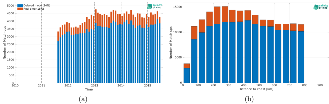
Figure 1: Number of match-ups between Argo and Aquarius SSS L3 OR v5 - Monthly - Rain mask (NASA-GSFC) SSS as a function of time (a) and as function of the distance to coast (b) over the SMOS coastal zone (<800km) 60N-60S Pi-MEP region and for the full satellite product period.
