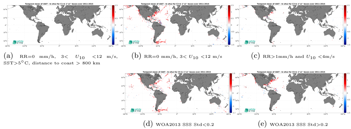
Figure 14: Temporal mean gridded over spatial boxes of size 1^\circ \times 1^\circ of \Delta\text{SSS} (Aquarius SSS L3 CAP v5 - 7-Day running (JPL) - TSG (SAMOS)) for 5 different subdatasets corresponding to: RR=0 mm/h, 3 < U_{10} < 12 m/s, SST > 5^\circ\text{C} , distance to coast > 800 km (a), RR=0 mm/h, 3 < U_{10} < 12 m/s (b), RR > 1 mm/h and U_{10} < 4 m/s (c), WOA2013 SSS Std < 0.2 (d), WOA2013 SSS Std > 0.2 (e).
