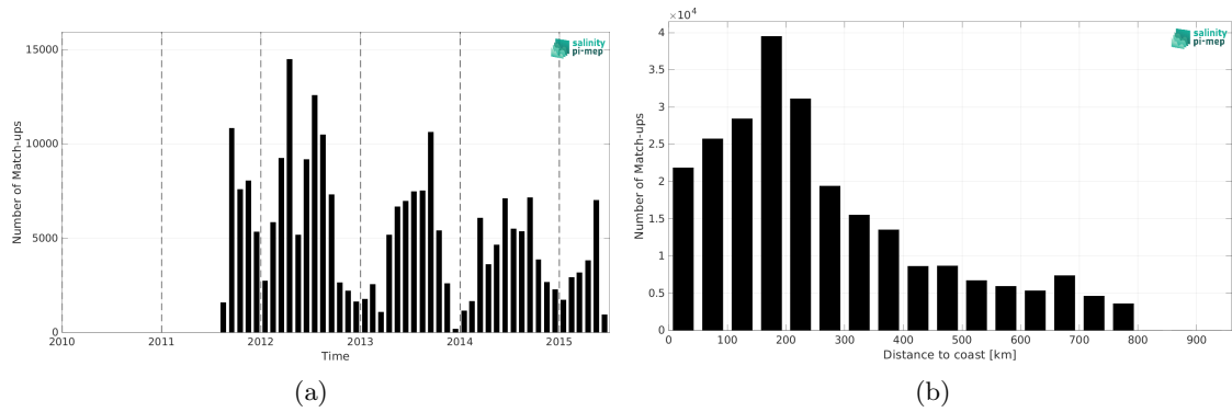
Figure 2: Number of match-ups between TSG (SAMOS) and Aquarius SSS L3 CAP v5 - 7-Day running (JPL) SSS as a function of time (a) and as function of the distance to coast (b) over the SMOS coastal zone (<800km) 60N-60S Pi-MEP region and for the full satellite product period.
