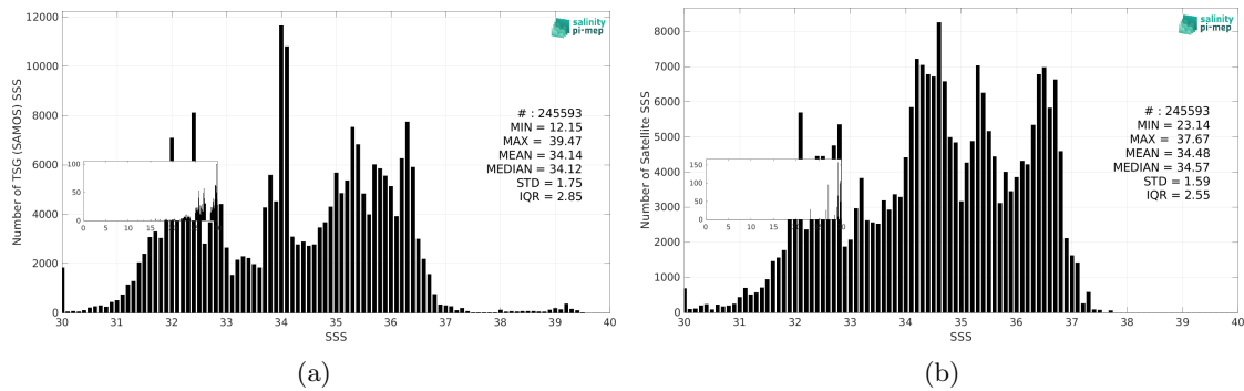
Figure 3: Histograms of SSS from TSG (SAMOS) (a) and Aquarius SSS L3 CAP v5 - 7-Day running (JPL) (b) considering all match-up pairs per bins of 0.1 over the SMOS coastal zone (<800km) 60N-60S Pi-MEP region and for the full satellite product period.
