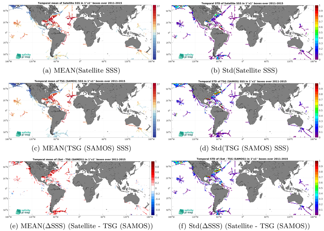
Figure 7: Temporal mean (left) and Std (right) of SSS from Aquarius SSS L3 CAP v5 - 7-Day running (JPL) (top), TSG (SAMOS) (middle), and of \Delta SSS (Satellite - TSG (SAMOS)). Only match-up pairs are used to generate these maps.
