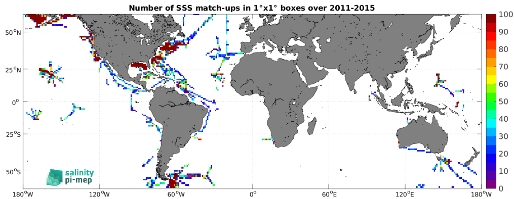
Figure 5: Number of SSS match-ups between TSG (SAMOS) SSS and the Aquarius SSS L3 CAP v5 - 7-Day running (JPL) SSS product for the SMOS coastal zone (<800km) 60N-60S Pi-MEP region over 1^\circ \times 1^\circ boxes and for the full satellite product period.
