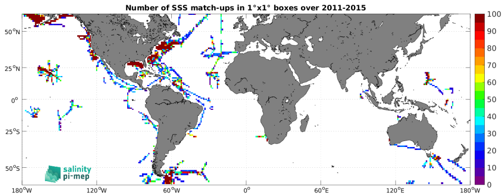
Figure 4: Number of SSS match-ups between TSG (SAMOS) SSS and the Aquarius SSS L3 CAP v5 - 7-Day running (JPL) SSS product for the SMOS coastal zone ( <800\text{km} ) 60N-60S Pi-MEP region over 1^\circ \times 1^\circ boxes and for the full satellite product period.
