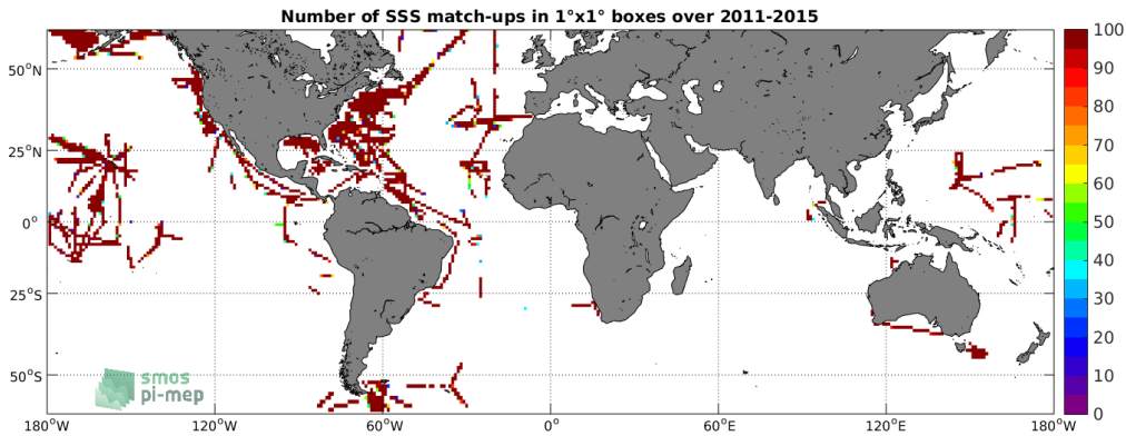
Figure 4: Number of SSS match-ups between TSG-SAMOS SSS and the Aquarius-L3-JPL-V5-7DAY-RUNNING SSS product for the SMOS coastal zone ( \pm 800\text{km} ) 60N-60S Pi-MEP region over 1^\circ \times 1^\circ boxes and for the full satellite product period.
