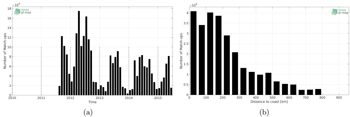
Figure 1: Number of match-ups between TSG-SAMOS and Aquarius-L3-JPL-V5-7DAY-RUNNING SSS as a function of time (a) and as function of the distance to coast (b) over the SMOS coastal zone ( \approx 800\text{km} ) 60N-60S Pi-MEP region and for the full satellite product period.
