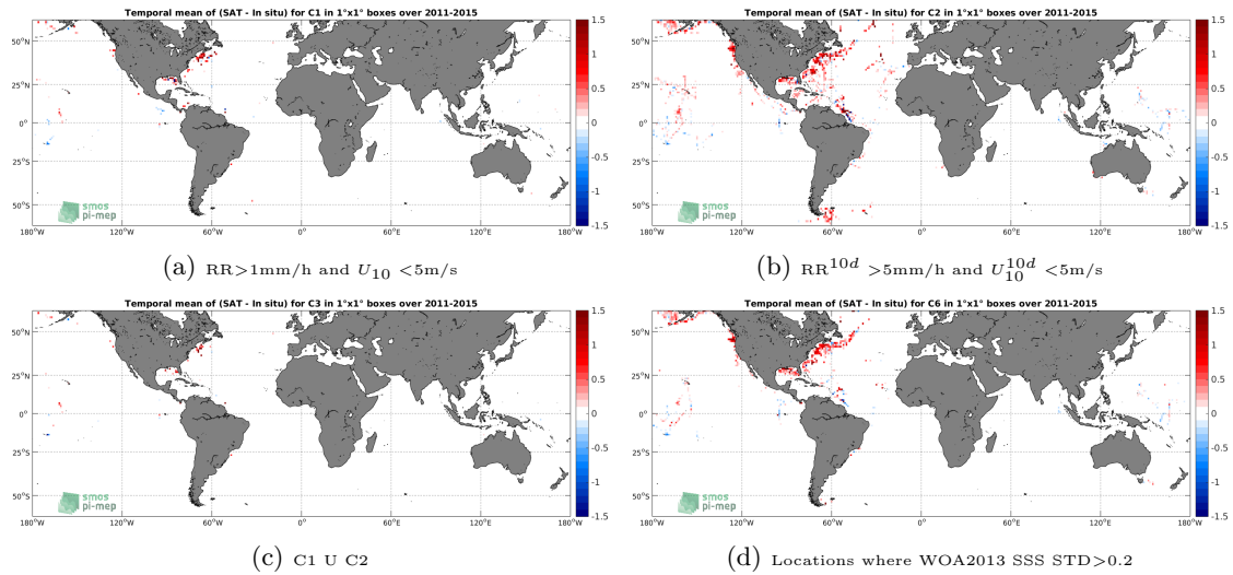
Figure 12: Temporal mean gridded over spatial boxes of size 1^\circ \times 1^\circ of \Delta SSS (Aquarius-L3-JPL-V5-7DAY-RUNNING - TSG-SAMOS) for 4 different subdatasets corresponding to: RR > 1\text{mm/h} and U_{10} < 5\text{m/s} (a), RR^{10d} > 5\text{mm/h} and U_{10}^{10d} < 5\text{m/s} (b), C1 U C2 (c), Locations where WOA2013 SSS STD > 0.2 (d).
