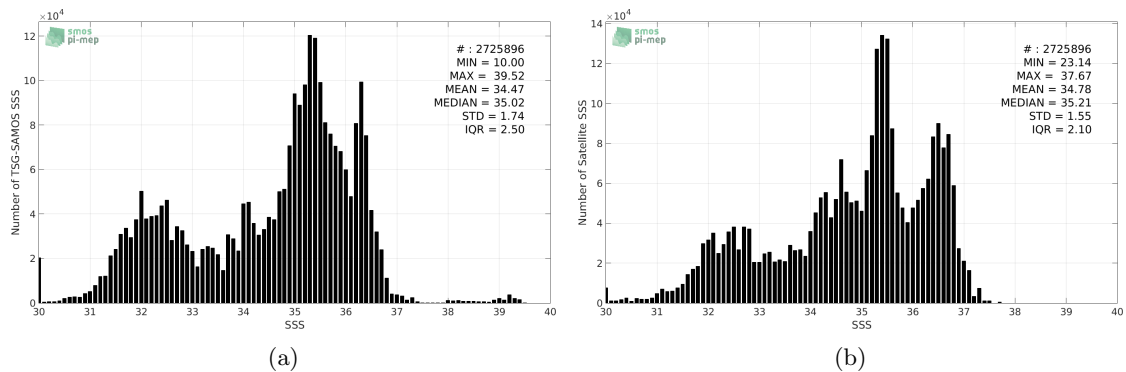
Figure 2: Histograms of SSS from TSG-SAMOS (a) and Aquarius-L3-JPL-V5-7DAY-RUNNING (b) considering all match-up pairs per bins of 0.1 over the SMOS coastal zone ( \approx 800\text{km} ) 60N-60S Pi-MEP region and for the full satellite product period.
