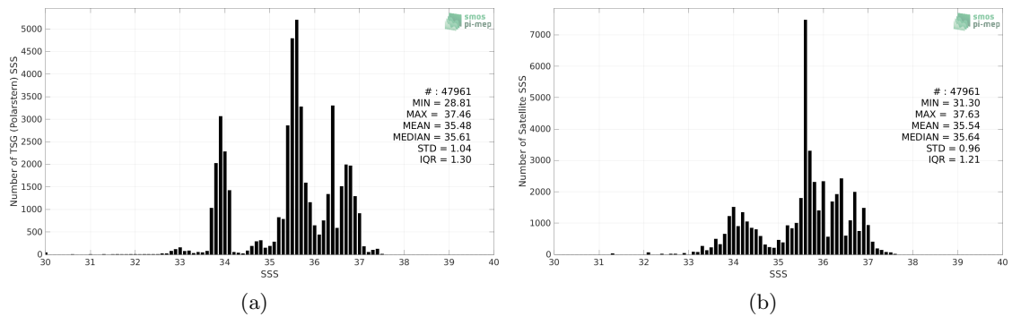
Figure 2: Histograms of SSS from TSG (Polarstern) (a) and Aquarius SSS L3 CAP v5 - 7-Day running (JPL) (b) considering all match-up pairs per bins of 0.1 over the SMOS coastal zone (<800km) 60N-60S Pi-MEP region and for the full satellite product period.
