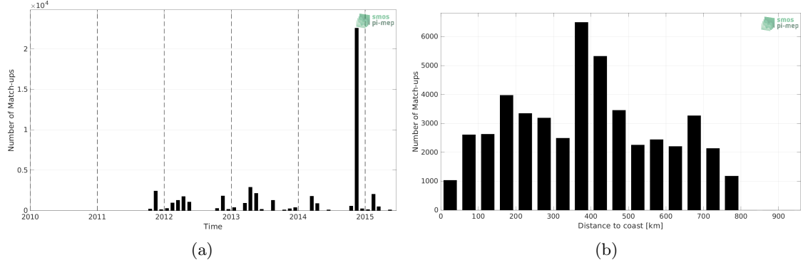
Figure 1: Number of match-ups between TSG (Polarstern) and Aquarius SSS L3 CAP v5 - 7-Day running (JPL) SSS as a function of time (a) and as function of the distance to coast (b) over the SMOS coastal zone ( <800\text{km} ) 60N-60S Pi-MEP region and for the full satellite product period.
