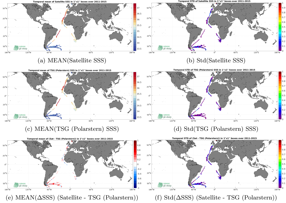
Figure 6: Temporal mean (left) and Std (right) of SSS from Aquarius SSS L3 CAP v5 - 7-Day running (JPL) (top), TSG (Polarstern) (middle), and of \Delta SSS (Satellite - TSG (Polarstern)). Only match-up pairs are used to generate these maps.
