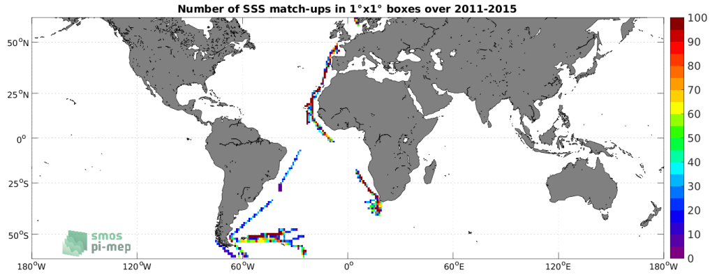
Figure 4: Number of SSS match-ups between TSG (Polarstern) SSS and the Aquarius SSS L3 CAP v5 - 7-Day running (JPL) SSS product for the SMOS coastal zone (<800km) 60N-60S Pi-MEP region over 1^\circ \times 1^\circ boxes and for the full satellite product period.
