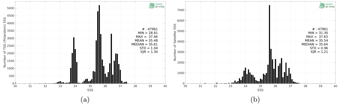
Figure 2: Histograms of SSS from TSG (Polarstern) (a) and Aquarius SSS L3 CAP v5 - 7-Day running (JPL) (b) considering all match-up pairs per bins of 0.1 over the SMOS coastal zone ( <800\text{km} ) 60N-60S Pi-MEP region and for the full satellite product period.
