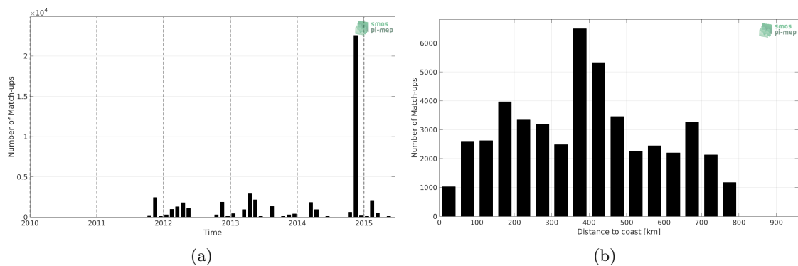
Figure 1: Number of match-ups between TSG-POLARSTERN and Aquarius-L3-JPL-V5-7DAY-RUNNING SSS as a function of time (a) and as function of the distance to coast (b) over the SMOS coastal zone ( \pm 800 km) 60N-60S Pi-MEP region and for the full satellite product period.
