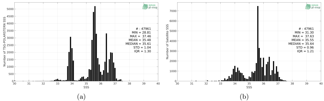
Figure 2: Histograms of SSS from TSG-POLARSTERN (a) and Aquarius-L3-JPL-V5-7DAY-RUNNING (b) considering all match-up pairs per bins of 0.1 over the SMOS coastal zone ( \pm 800\text{km} ) 60N-60S Pi-MEP region and for the full satellite product period.
