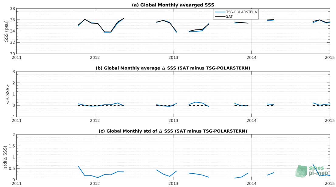
Figure 7: Time series of the monthly averaged mean SSS (top), mean \Delta SSS (Satellite - TSG-POLARSTERN) and Std of \Delta SSS (Satellite - TSG-POLARSTERN) over the SMOS coastal zone ( \approx 800\text{km} ) 60N-60S Pi-MEP region considering all match-ups collected by the Pi-MEP platform.
