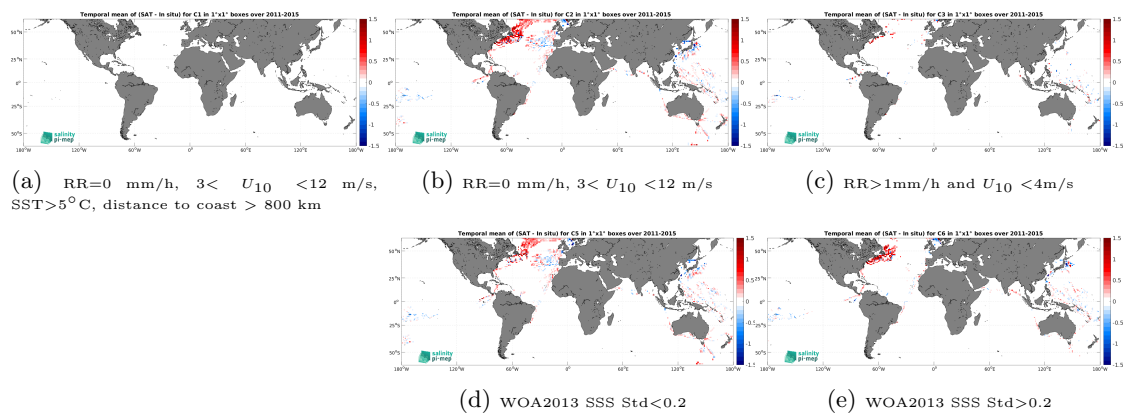
Figure 14: Temporal mean gridded over spatial boxes of size 1^\circ \times 1^\circ of \Delta SSS (Aquarius SSS L3 CAP v5 - 7-Day running (JPL) - TSG (LEGOS-DM)) for 5 different subdatasets corresponding to:RR=0 mm/h, 3 < U_{10} < 12 m/s, SST >5^\circ\text{C} , distance to coast > 800 km (a), RR=0 mm/h, 3 < U_{10} < 12 m/s (b), RR >1 mm/h and U_{10} < 4 m/s (c), WOA2013 SSS Std <0.2 (d), WOA2013 SSS Std >0.2 (e).
