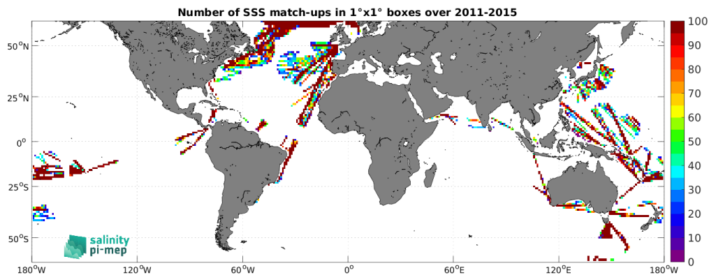
Figure 5: Number of SSS match-ups between TSG (LEGOS-DM) SSS and the Aquarius SSS L3 CAP v5 - 7-Day running (JPL) SSS product for the SMOS coastal zone (<800km) 60N-60S Pi-MEP region over 1^\circ \times 1^\circ boxes and for the full satellite product period.
