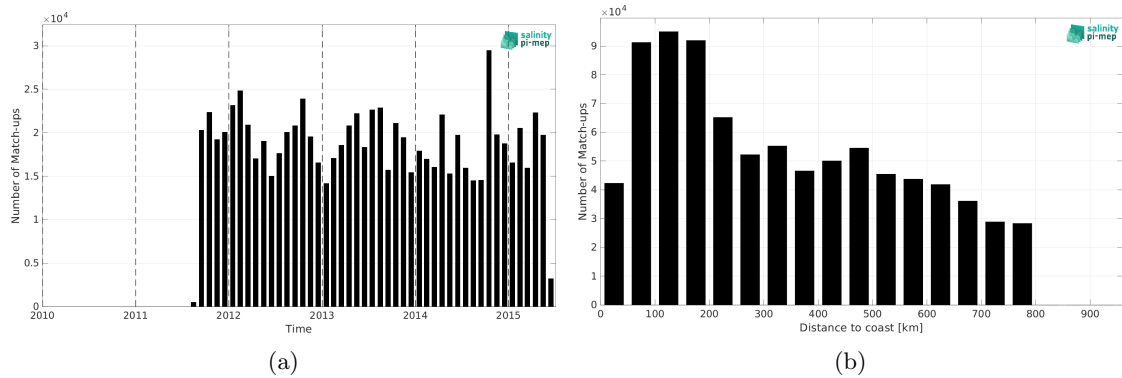
Figure 2: Number of match-ups between TSG (LEGOS-DM) and Aquarius SSS L3 CAP v5 - 7-Day running (JPL) SSS as a function of time (a) and as function of the distance to coast (b) over the SMOS coastal zone (<800km) 60N-60S Pi-MEP region and for the full satellite product period.
