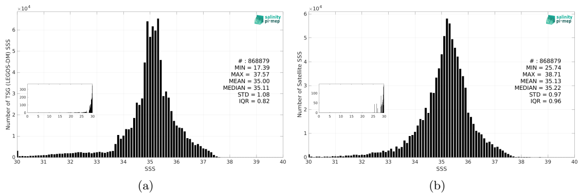
Figure 3: Histograms of SSS from TSG (LEGOS-DM) (a) and Aquarius SSS L3 CAP v5 - 7-Day running (JPL) (b) considering all match-up pairs per bins of 0.1 over the SMOS coastal zone (<800km) 60N-60S Pi-MEP region and for the full satellite product period.
