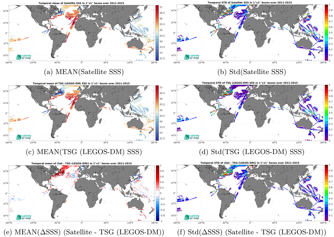
Figure 7: Temporal mean (left) and Std (right) of SSS from Aquarius SSS L3 CAP v5 - 7-Day running (JPL) (top), TSG (LEGOS-DM) (middle), and of \Delta SSS (Satellite - TSG (LEGOS-DM)). Only match-up pairs are used to generate these maps.
