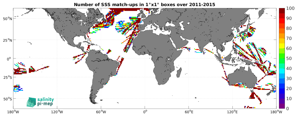
Figure 4: Number of SSS match-ups between TSG (LEGOS-DM) SSS and the Aquarius SSS L3 CAP v5 - 7-Day running (JPL) SSS product for the SMOS coastal zone (<800km) 60N-60S Pi-MEP region over 1^\circ \times 1^\circ boxes and for the full satellite product period.
