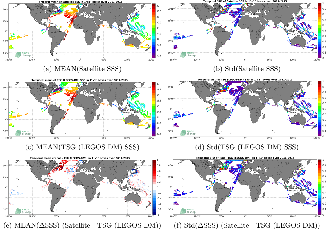
Figure 6: Temporal mean (left) and Std (right) of SSS from Aquarius SSS L3 CAP v5 - 7-Day running (JPL) (top), TSG (LEGOS-DM) (middle), and of \Delta SSS (Satellite - TSG (LEGOS-DM)). Only match-up pairs are used to generate these maps.
