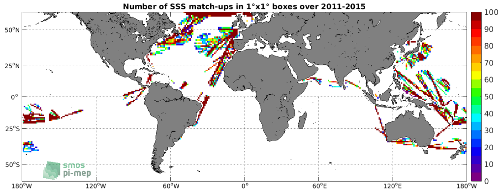
Figure 4: Number of SSS match-ups between TSG (LEGOS-DM) SSS and the Aquarius SSS L3 CAP v5 - 7-Day running (JPL) SSS product for the SMOS coastal zone (<800km) 60N-60S Pi-MEP region over 1°x1° boxes and for the full satellite product period.
