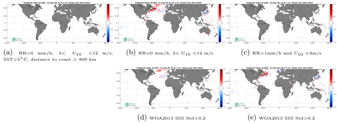
Figure 12: Temporal mean gridded over spatial boxes of size 1^\circ \times 1^\circ of \Delta SSS (Aquarius SSS L3 CAP v5 - 7-Day running (JPL) - TSG (LEGOS-DM)) for 5 different subdatasets corresponding to:RR=0 mm/h, 3 < U_{10} < 12 m/s, SST >5^\circ C, distance to coast > 800 km (a), RR=0 mm/h, 3 < U_{10} < 12 m/s (b), RR >1 mm/h and U_{10} < 4 m/s (c), WOA2013 SSS Std <0.2 (d), WOA2013 SSS Std >0.2 (e).
