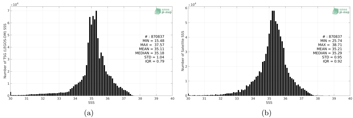
Figure 2: Histograms of SSS from TSG (LEGOS-DM) (a) and Aquarius SSS L3 CAP v5 - 7-Day running (JPL) (b) considering all match-up pairs per bins of 0.1 over the SMOS coastal zone (<800km) 60N-60S Pi-MEP region and for the full satellite product period.
