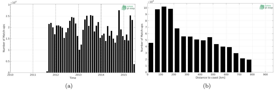
Figure 1: Number of match-ups between TSG (LEGOS-DM) and Aquarius SSS L3 CAP v5 - 7-Day running (JPL) SSS as a function of time (a) and as function of the distance to coast (b) over the SMOS coastal zone (<800km) 60N-60S Pi-MEP region and for the full satellite product period.
